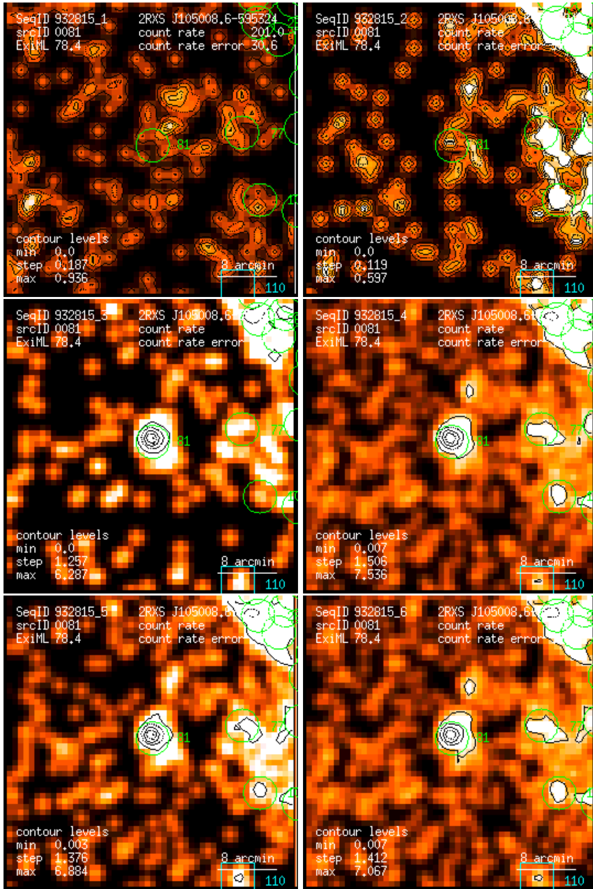
Figure 81: RASS 932815: detection 0081: band rate images, Gaussian filter: (1) PSPC channels 11 – 41, (2) 52 – 90, (3) 91 – 201, (4) 11 – 235, (5) 52 – 201, (6) 11 – 201. Broad band rates in counts/ks. Band rate contour levels in counts/ks/arcmin 2 .
