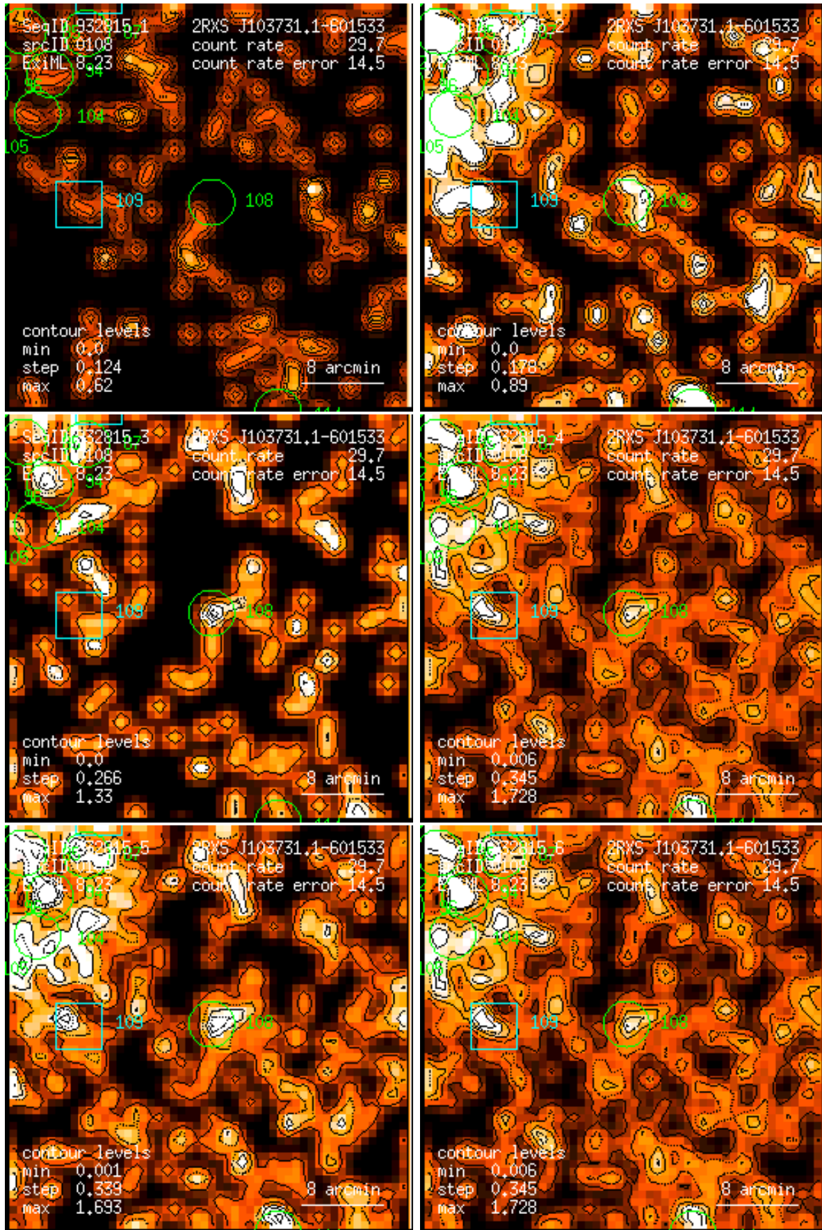
Figure 108: RASS 932815: detection 0108: band rate images, Gaussian filter: (1) PSPC channels 11 – 41, (2) 52 – 90, (3) 91 – 201, (4) 11 – 235, (5) 52 – 201, (6) 11 – 201. Broad band rates in counts/ks. Band rate contour levels in counts/ks/arcmin 2 .
