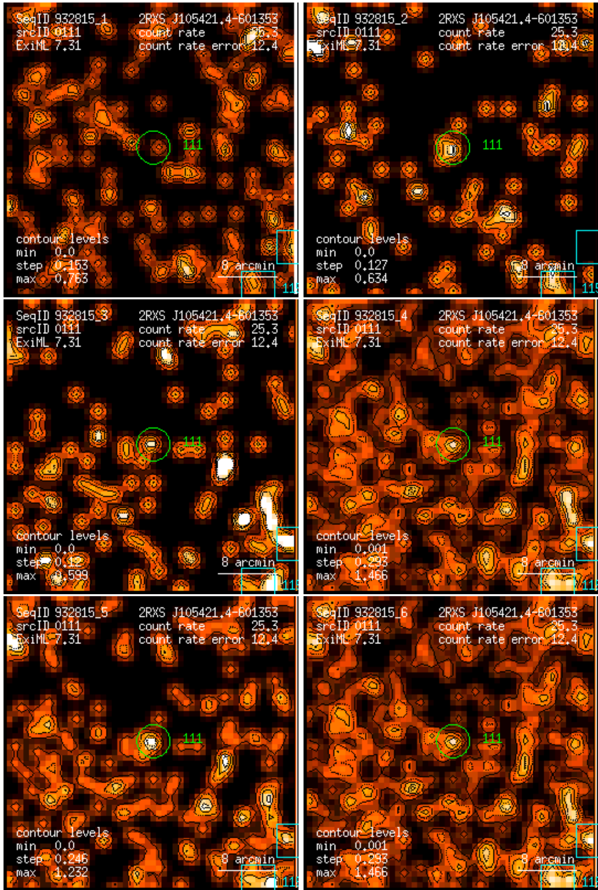
Figure 111: RASS 932815: detection 0111: band rate images, Gaussian filter: (1) PSPC channels 11 – 41, (2) 52 – 90, (3) 91 – 201, (4) 11 – 235, (5) 52 – 201, (6) 11 – 201. Broad band rates in counts/ks. Band rate contour levels in counts/ks/arcmin 2 .
