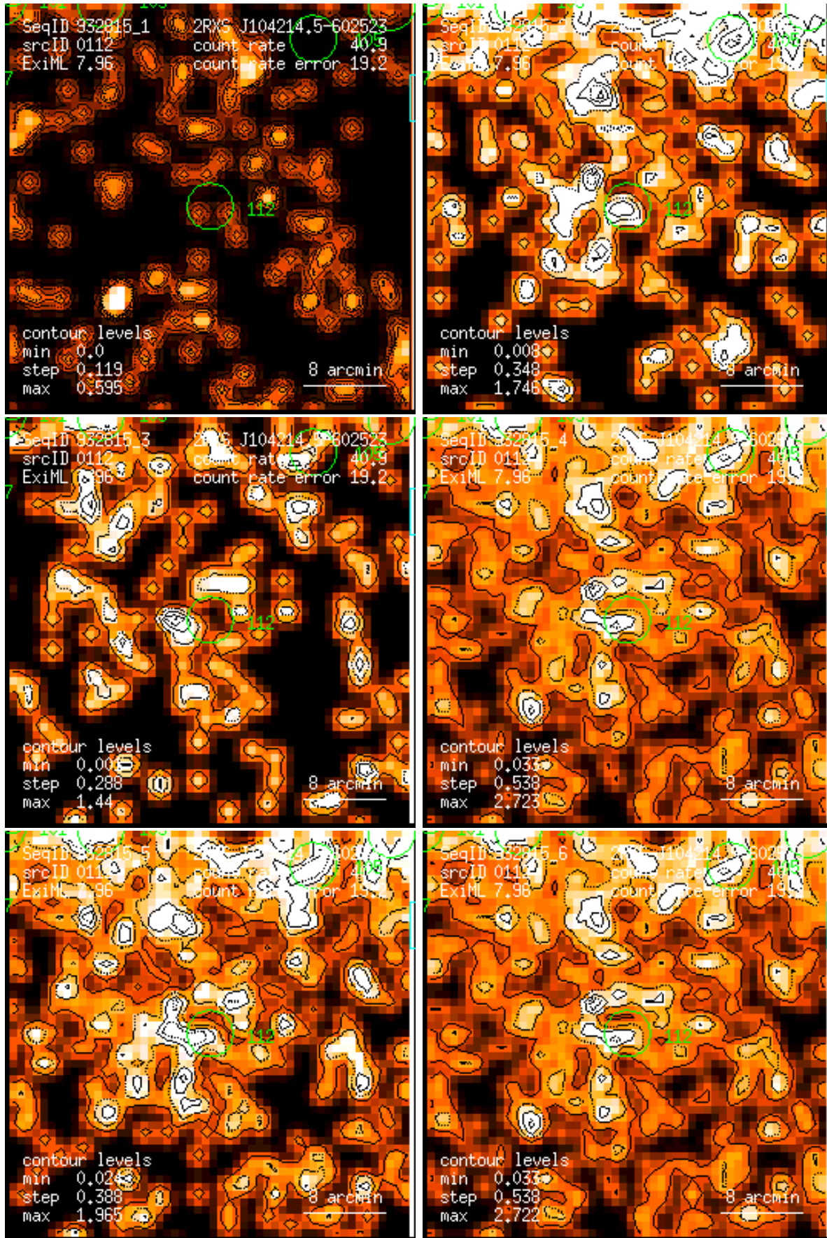
Figure 112: RASS 932815: detection 0112: band rate images, Gaussian filter: (1) PSPC channels 11 – 41, (2) 52 – 90, (3) 91 – 201, (4) 11 – 235, (5) 52 – 201, (6) 11 – 201. Broad band rates in counts/ks. Band rate contour levels in counts/ks/arcmin 2 .
