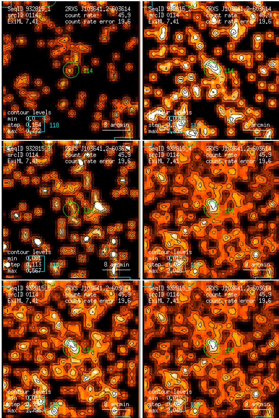
Figure 114: RASS 932815: detection 0114: band rate images, Gaussian filter: (1) PSPC channels 11 – 41, (2) 52 – 90, (3) 91 – 201, (4) 11 – 235, (5) 52 – 201, (6) 11 – 201. Broad band rates in counts/ks. Band rate contour levels in counts/ks/arcmin 2 .
