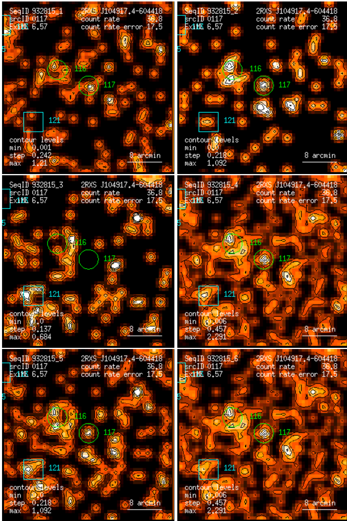
Figure 117: RASS 932815: detection 0117: band rate images, Gaussian filter: (1) PSPC channels 11 – 41, (2) 52 – 90, (3) 91 – 201, (4) 11 – 235, (5) 52 – 201, (6) 11 – 201. Broad band rates in counts/ks. Band rate contour levels in counts/ks/arcmin 2 .
