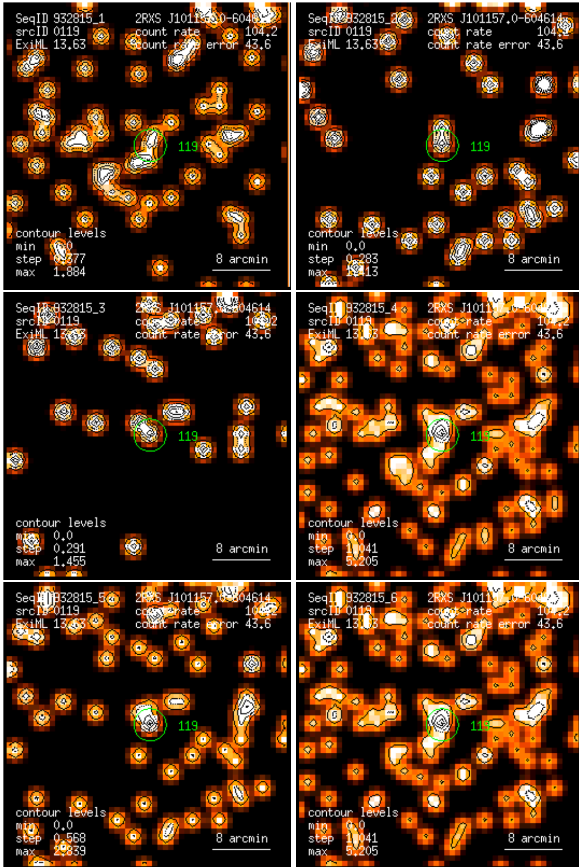
Figure 119: RASS 932815: detection 0119: band rate images, Gaussian filter: (1) PSPC channels 11 – 41, (2) 52 – 90, (3) 91 – 201, (4) 11 – 235, (5) 52 – 201, (6) 11 – 201. Broad band rates in counts/ks. Band rate contour levels in counts/ks/arcmin 2 .
