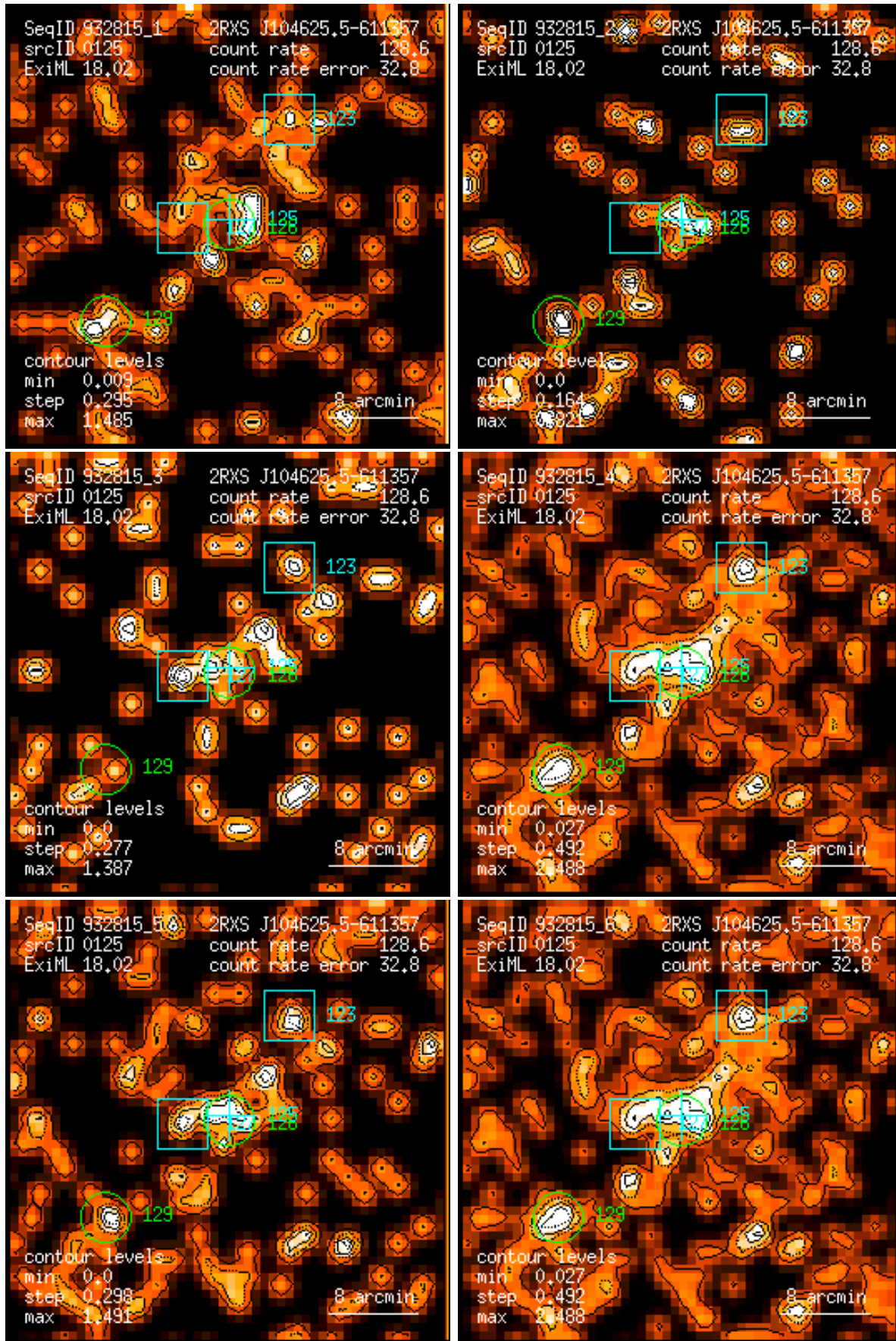
Figure 125: RASS 932815: detection 0125: band rate images, Gaussian filter: (1) PSPC channels 11 – 41, (2) 52 – 90, (3) 91 – 201, (4) 11 – 235, (5) 52 – 201, (6) 11 – 201. Broad band rates in counts/ks. Band rate contour levels in counts/ks/arcmin 2 .
