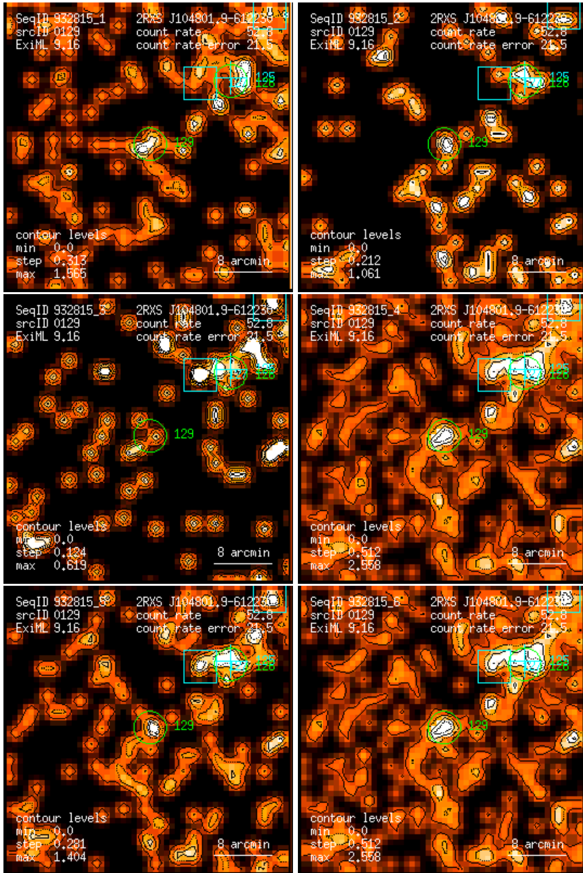
Figure 129: RASS 932815: detection 0129: band rate images, Gaussian filter: (1) PSPC channels 11 – 41, (2) 52 – 90, (3) 91 – 201, (4) 11 – 235, (5) 52 – 201, (6) 11 – 201. Broad band rates in counts/ks. Band rate contour levels in counts/ks/arcmin 2 .
