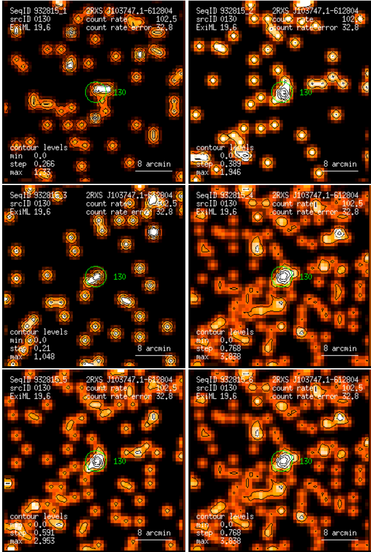
Figure 130: RASS 932815: detection 0130: band rate images, Gaussian filter: (1) PSPC channels 11 – 41, (2) 52 – 90, (3) 91 – 201, (4) 11 – 235, (5) 52 – 201, (6) 11 – 201. Broad band rates in counts/ks. Band rate contour levels in counts/ks/arcmin 2 .
