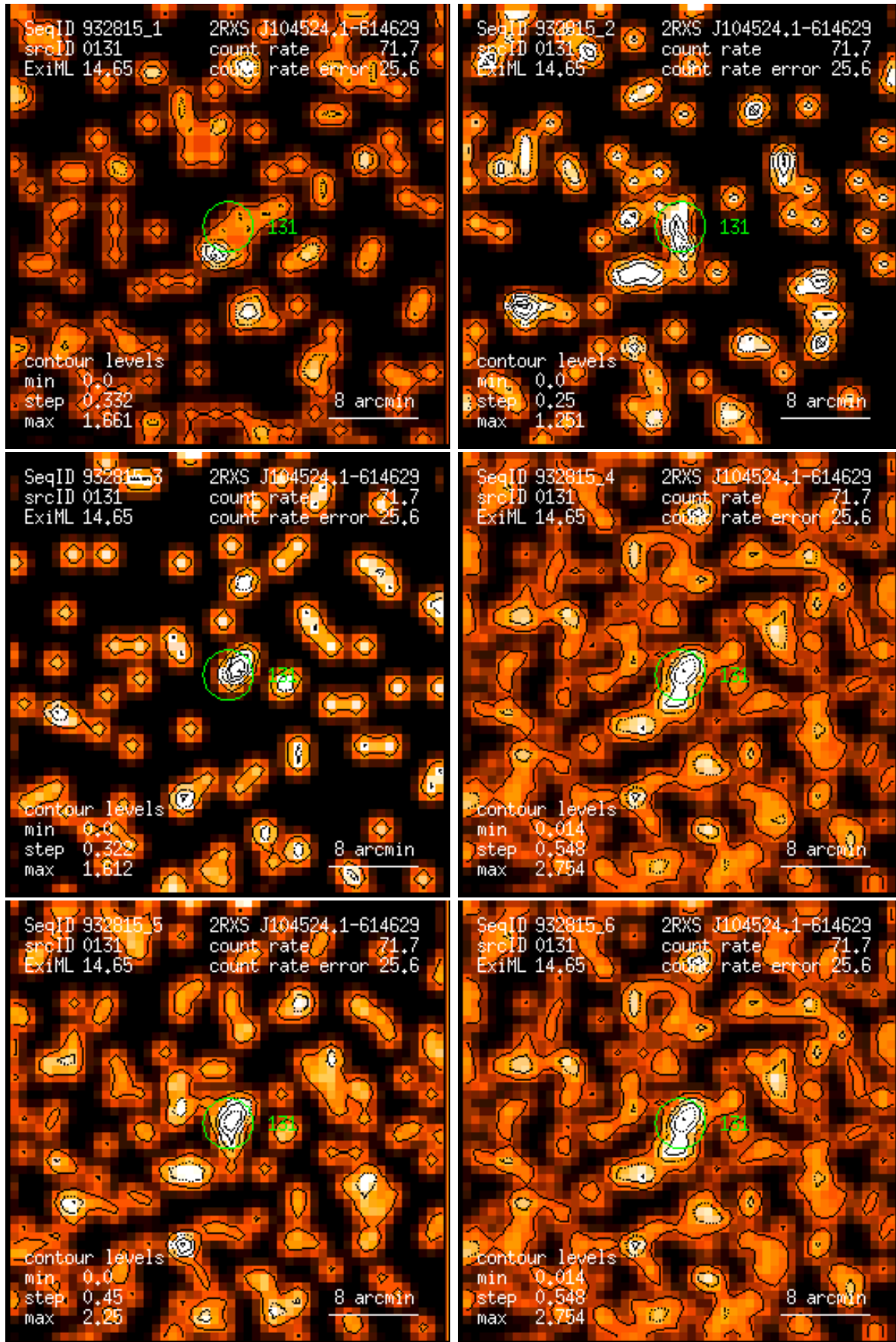
Figure 131: RASS 932815: detection 0131: band rate images, Gaussian filter: (1) PSPC channels 11 – 41, (2) 52 – 90, (3) 91 – 201, (4) 11 – 235, (5) 52 – 201, (6) 11 – 201. Broad band rates in counts/ks. Band rate contour levels in counts/ks/arcmin 2 .
