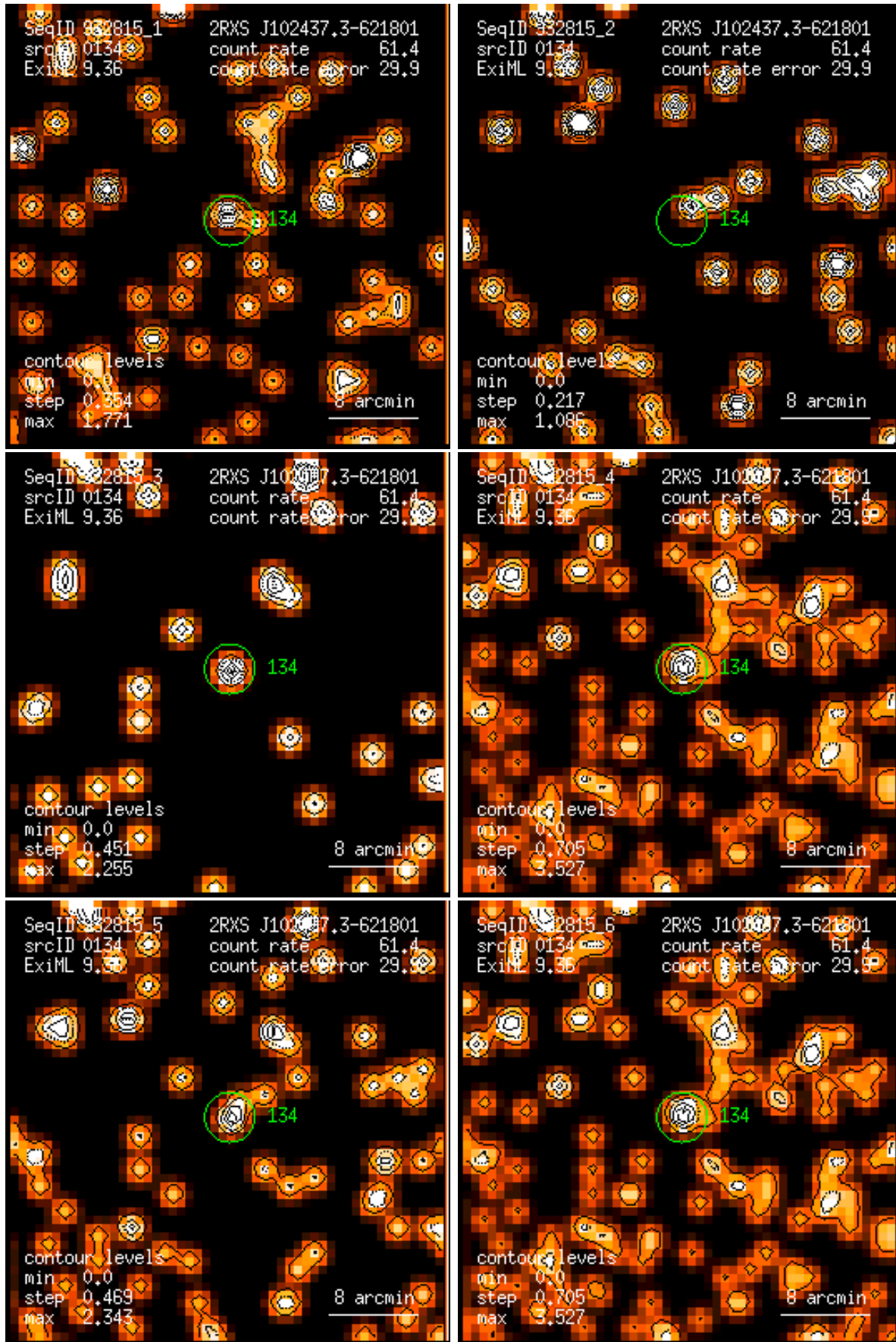
Figure 134: RASS 932815: detection 0134: band rate images, Gaussian filter: (1) PSPC channels 11 – 41, (2) 52 – 90, (3) 91 – 201, (4) 11 – 235, (5) 52 – 201, (6) 11 – 201. Broad band rates in counts/ks. Band rate contour levels in counts/ks/arcmin 2 .
