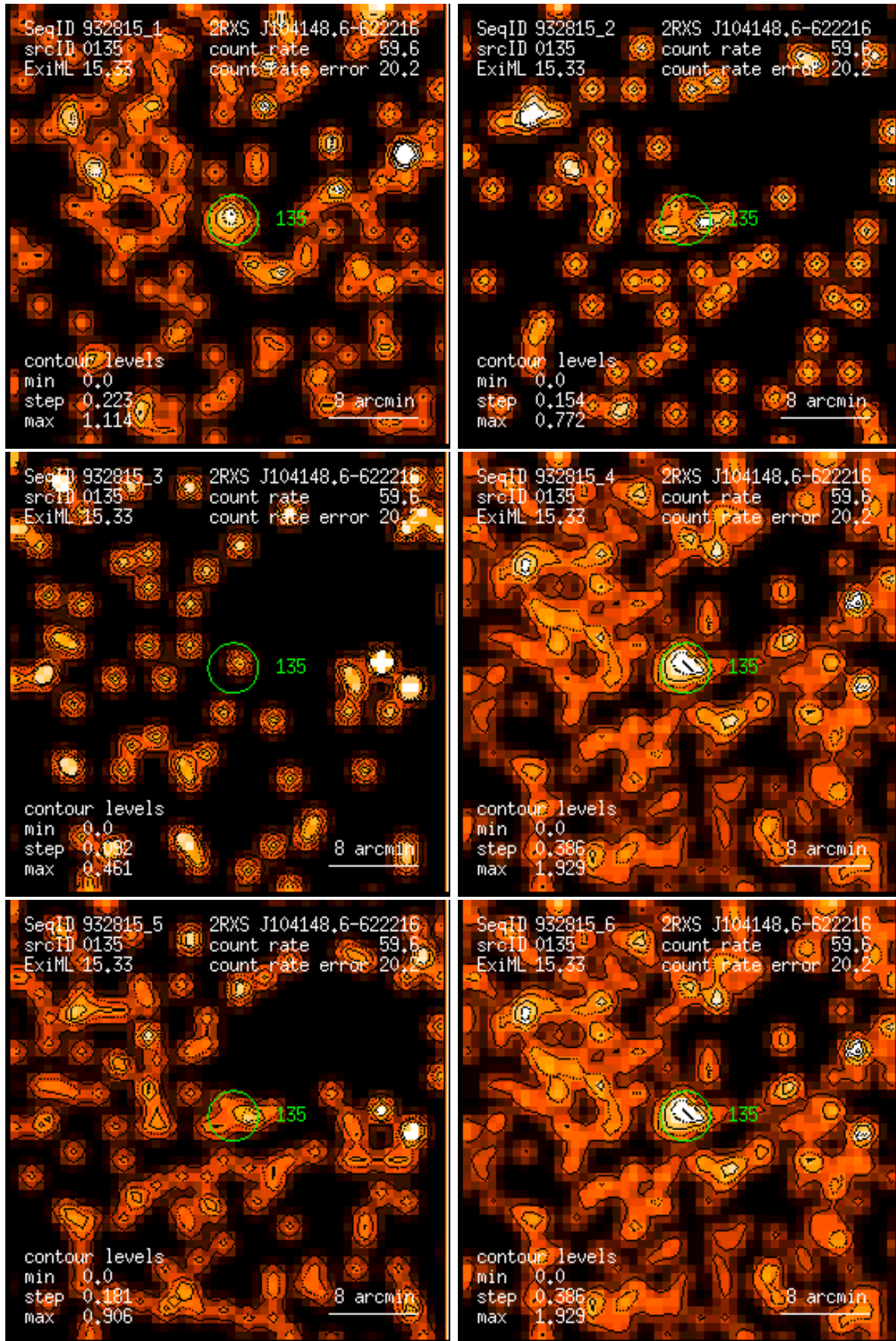
Figure 135: RASS 932815: detection 0135: band rate images, Gaussian filter: (1) PSPC channels 11 – 41, (2) 52 – 90, (3) 91 – 201, (4) 11 – 235, (5) 52 – 201, (6) 11 – 201. Broad band rates in counts/ks. Band rate contour levels in counts/ks/arcmin 2 .
