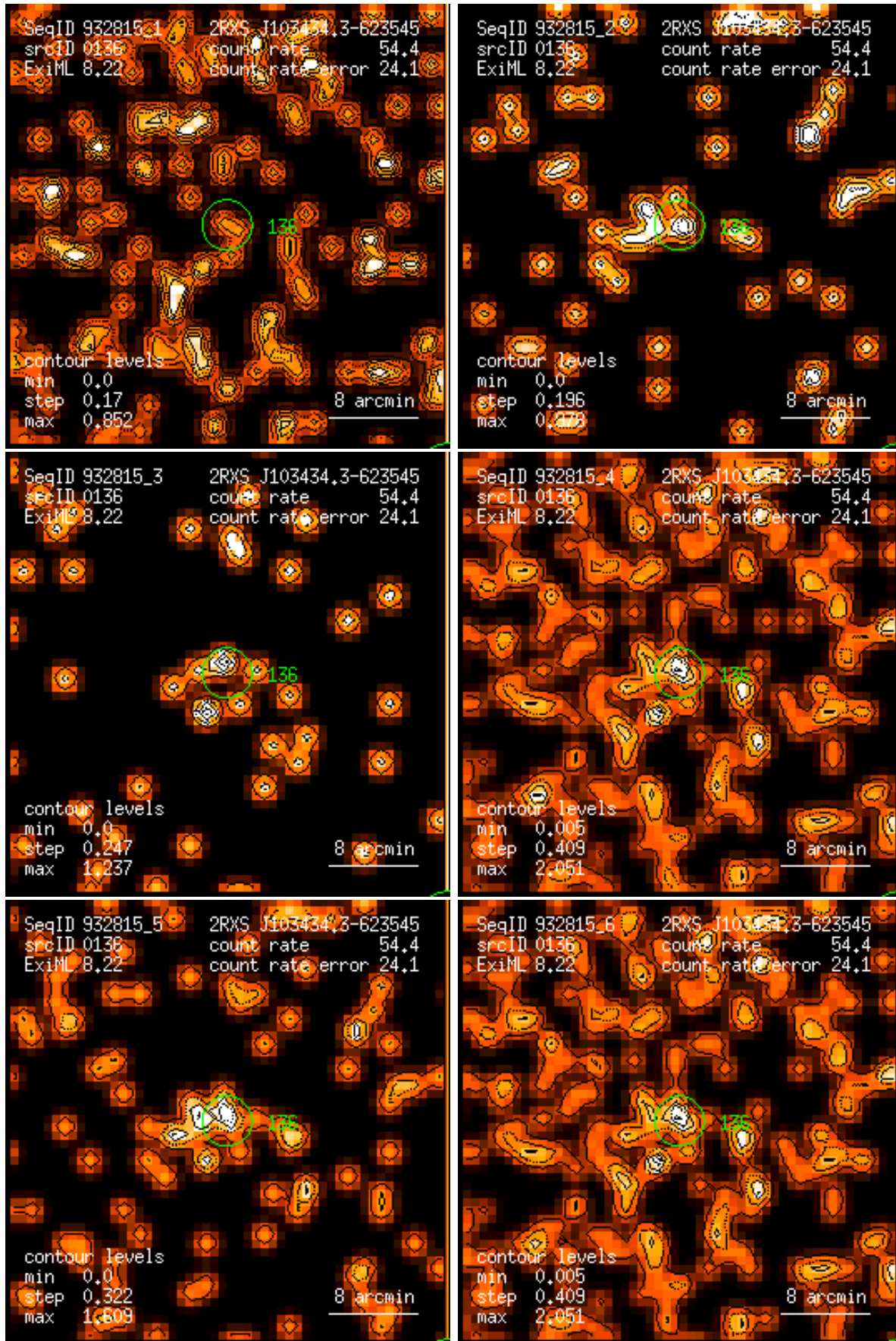
Figure 136: RASS 932815: detection 0136: band rate images, Gaussian filter: (1) PSPC channels 11 – 41, (2) 52 – 90, (3) 91 – 201, (4) 11 – 235, (5) 52 – 201, (6) 11 – 201. Broad band rates in counts/ks. Band rate contour levels in counts/ks/arcmin 2 .
