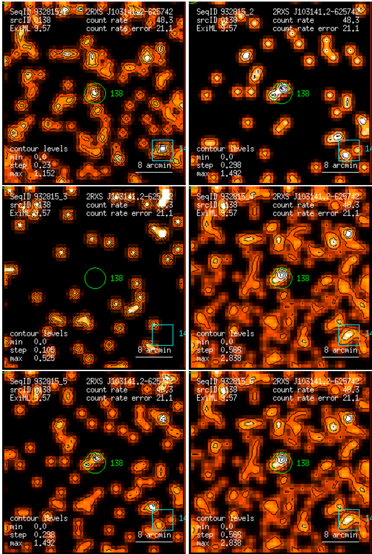
Figure 138: RASS 932815: detection 0138: band rate images, Gaussian filter: (1) PSPC channels 11 – 41, (2) 52 – 90, (3) 91 – 201, (4) 11 – 235, (5) 52 – 201, (6) 11 – 201. Broad band rates in counts/ks. Band rate contour levels in counts/ks/arcmin 2 .
