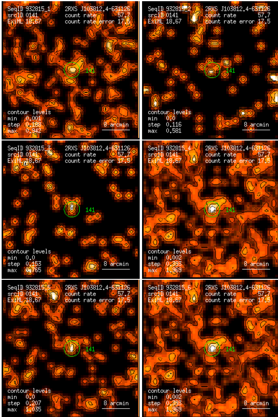
Figure 141: RASS 932815: detection 0141: band rate images, Gaussian filter: (1) PSPC channels 11 – 41, (2) 52 – 90, (3) 91 – 201, (4) 11 – 235, (5) 52 – 201, (6) 11 – 201. Broad band rates in counts/ks. Band rate contour levels in counts/ks/arcmin 2 .
