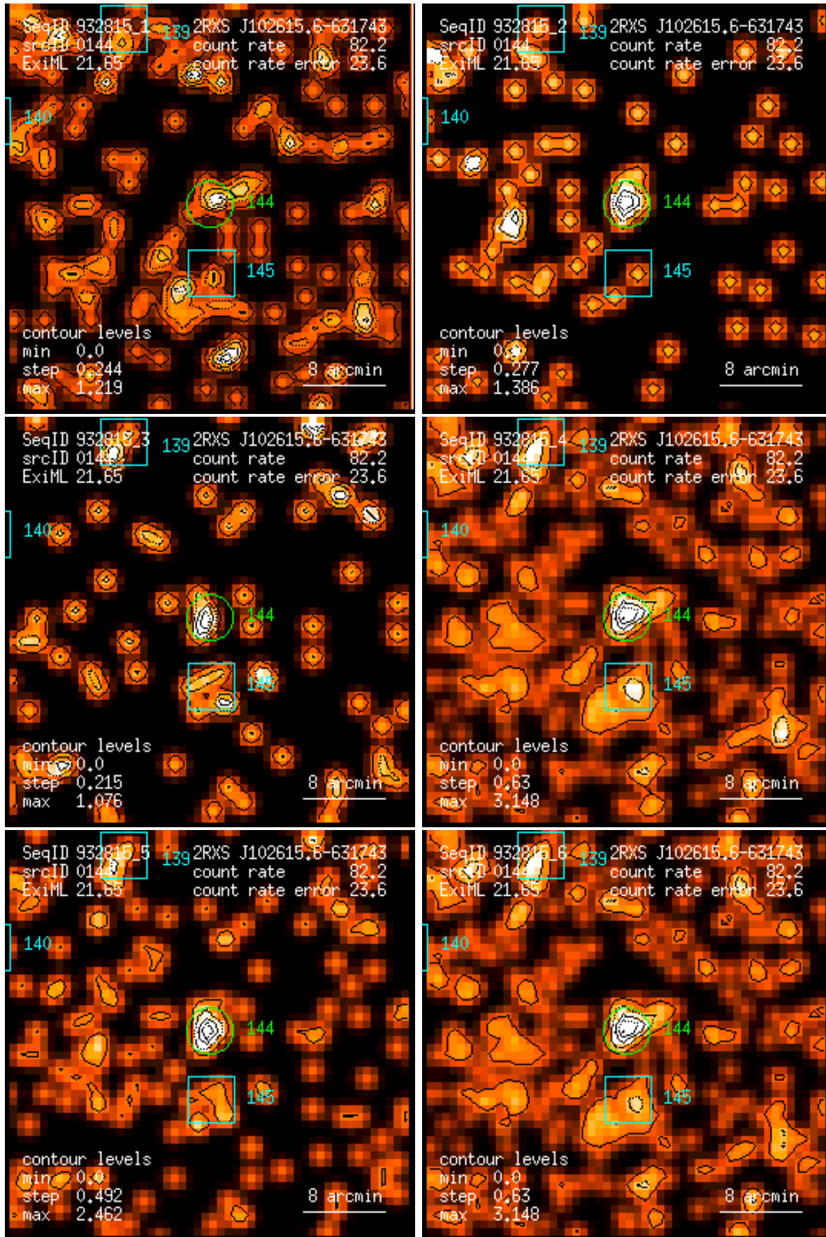
Figure 144: RASS 932815: detection 0144: band rate images, Gaussian filter: (1) PSPC channels 11 – 41, (2) 52 – 90, (3) 91 – 201, (4) 11 – 235, (5) 52 – 201, (6) 11 – 201. Broad band rates in counts/ks. Band rate contour levels in counts/ks/arcmin 2 .
