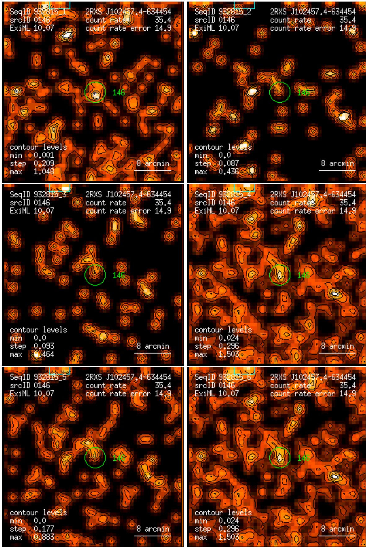
Figure 146: RASS 932815: detection 0146: band rate images, Gaussian filter: (1) PSPC channels 11 – 41, (2) 52 – 90, (3) 91 – 201, (4) 11 – 235, (5) 52 – 201, (6) 11 – 201. Broad band rates in counts/ks. Band rate contour levels in counts/ks/arcmin 2 .
