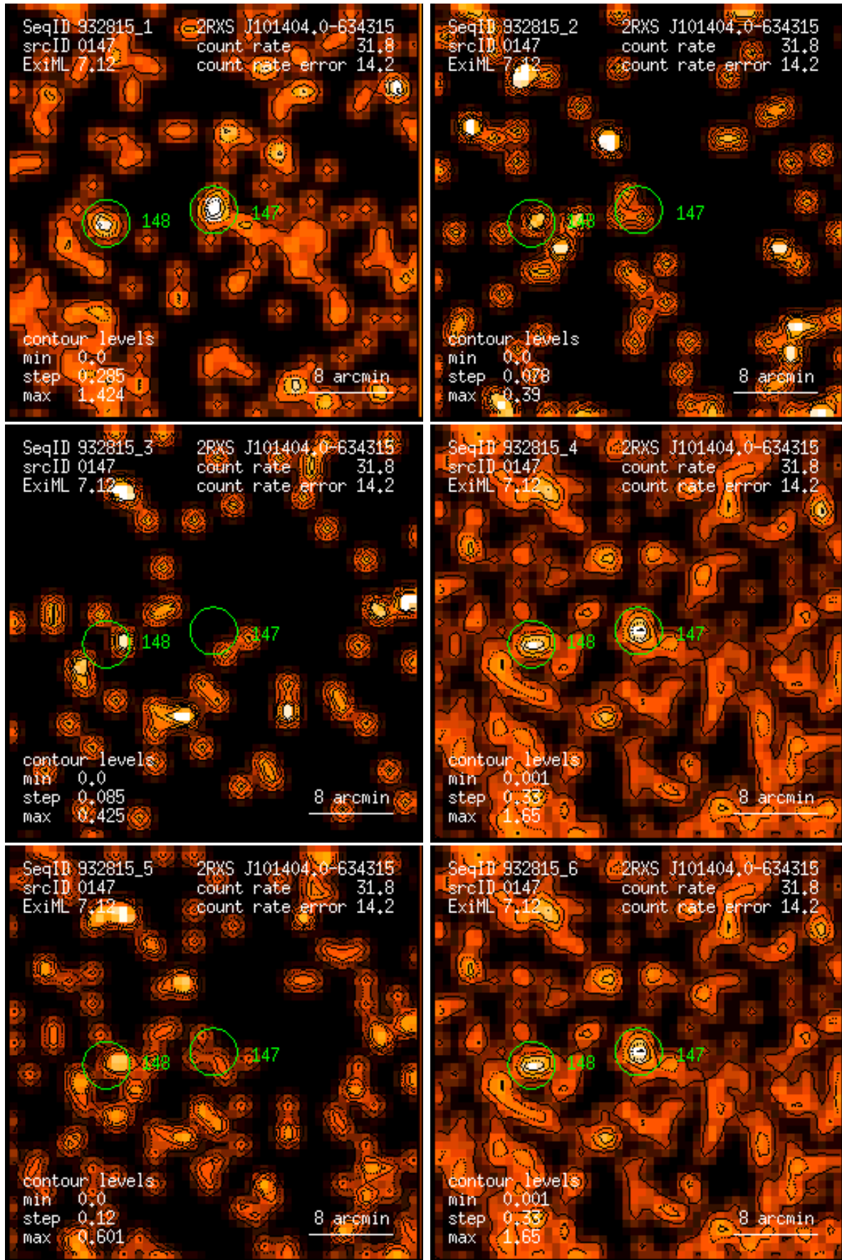
Figure 147: RASS 932815: detection 0147: band rate images, Gaussian filter: (1) PSPC channels 11 – 41, (2) 52 – 90, (3) 91 – 201, (4) 11 – 235, (5) 52 – 201, (6) 11 – 201. Broad band rates in counts/ks. Band rate contour levels in counts/ks/arcmin 2 .
