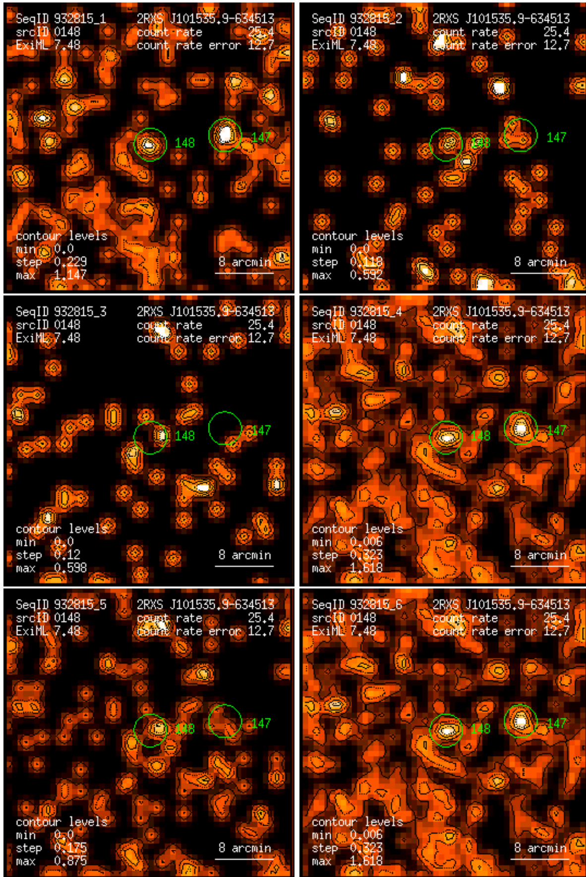
Figure 148: RASS 932815: detection 0148: band rate images, Gaussian filter: (1) PSPC channels 11 – 41, (2) 52 – 90, (3) 91 – 201, (4) 11 – 235, (5) 52 – 201, (6) 11 – 201. Broad band rates in counts/ks. Band rate contour levels in counts/ks/arcmin 2 .
