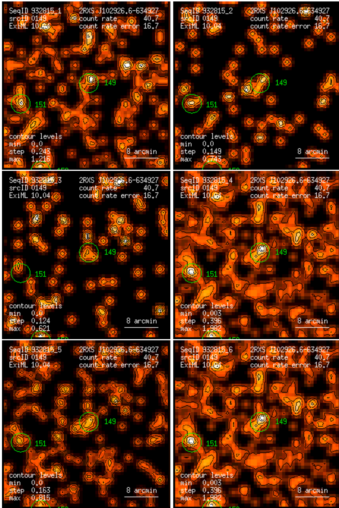
Figure 149: RASS 932815: detection 0149: band rate images, Gaussian filter: (1) PSPC channels 11 – 41, (2) 52 – 90, (3) 91 – 201, (4) 11 – 235, (5) 52 – 201, (6) 11 – 201. Broad band rates in counts/ks. Band rate contour levels in counts/ks/arcmin 2 .
