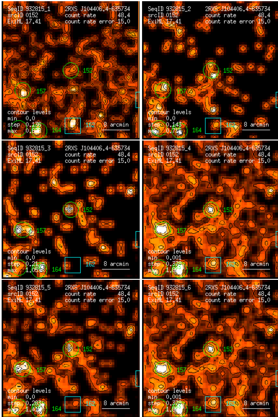
Figure 152: RASS 932815: detection 0152: band rate images, Gaussian filter: (1) PSPC channels 11 – 41, (2) 52 – 90, (3) 91 – 201, (4) 11 – 235, (5) 52 – 201, (6) 11 – 201. Broad band rates in counts/ks. Band rate contour levels in counts/ks/arcmin 2 .
