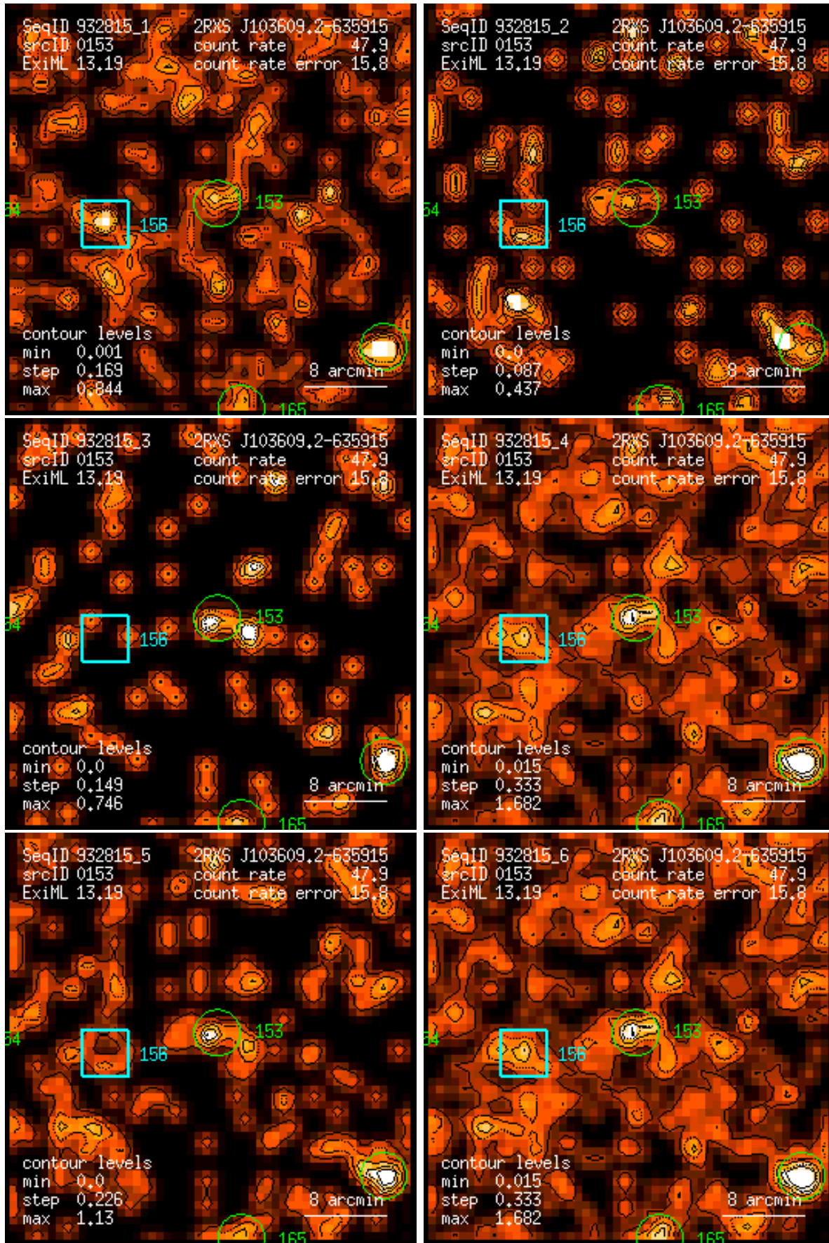
Figure 153: RASS 932815: detection 0153: band rate images, Gaussian filter: (1) PSPC channels 11 – 41, (2) 52 – 90, (3) 91 – 201, (4) 11 – 235, (5) 52 – 201, (6) 11 – 201. Broad band rates in counts/ks. Band rate contour levels in counts/ks/arcmin 2 .
