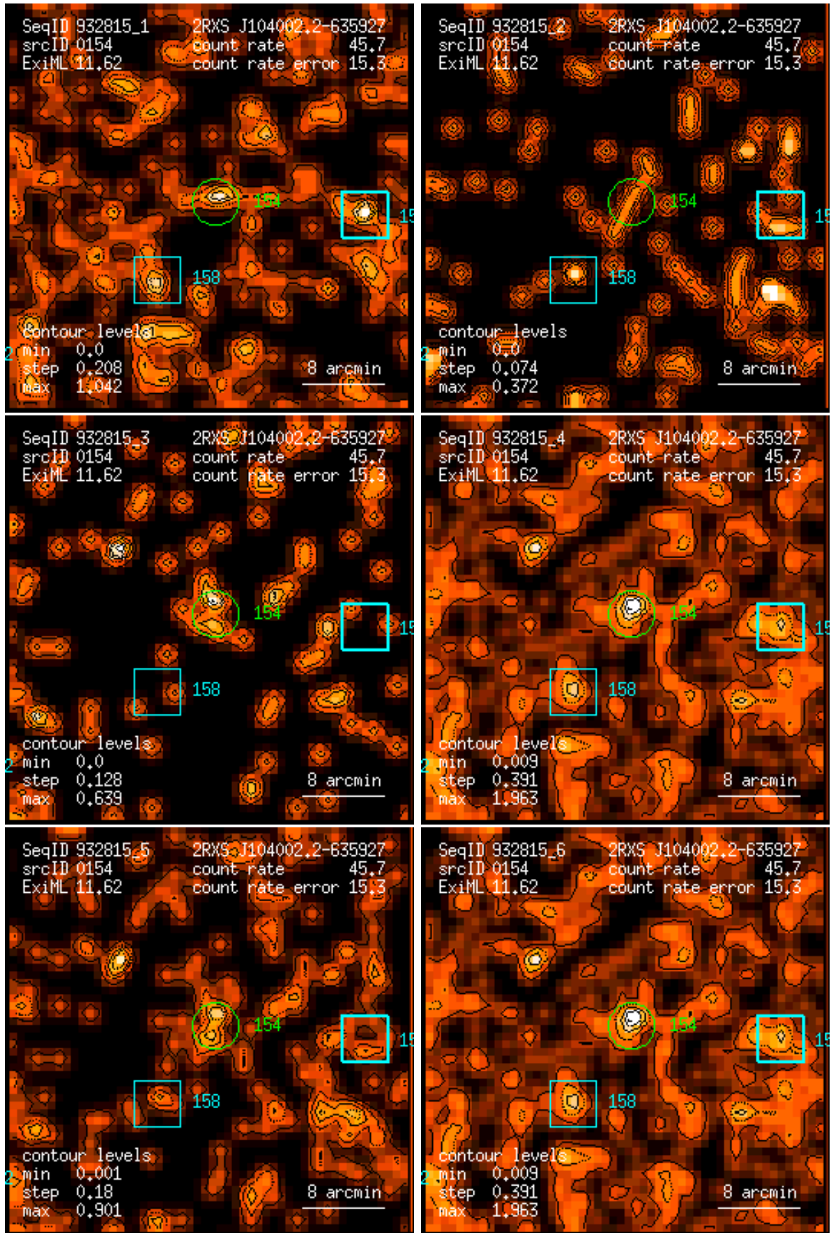
Figure 154: RASS 932815: detection 0154: band rate images, Gaussian filter: (1) PSPC channels 11 – 41, (2) 52 – 90, (3) 91 – 201, (4) 11 – 235, (5) 52 – 201, (6) 11 – 201. Broad band rates in counts/ks. Band rate contour levels in counts/ks/arcmin 2 .
