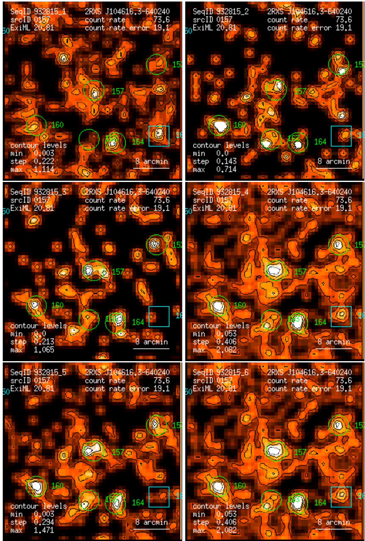
Figure 157: RASS 932815: detection 0157: band rate images, Gaussian filter: (1) PSPC channels 11 – 41, (2) 52 – 90, (3) 91 – 201, (4) 11 – 235, (5) 52 – 201, (6) 11 – 201. Broad band rates in counts/ks. Band rate contour levels in counts/ks/arcmin 2 .
