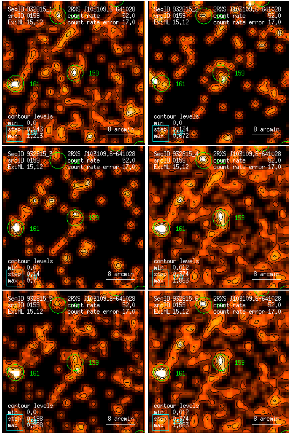
Figure 159: RASS 932815: detection 0159: band rate images, Gaussian filter: (1) PSPC channels 11 – 41, (2) 52 – 90, (3) 91 – 201, (4) 11 – 235, (5) 52 – 201, (6) 11 – 201. Broad band rates in counts/ks. Band rate contour levels in counts/ks/arcmin 2 .
