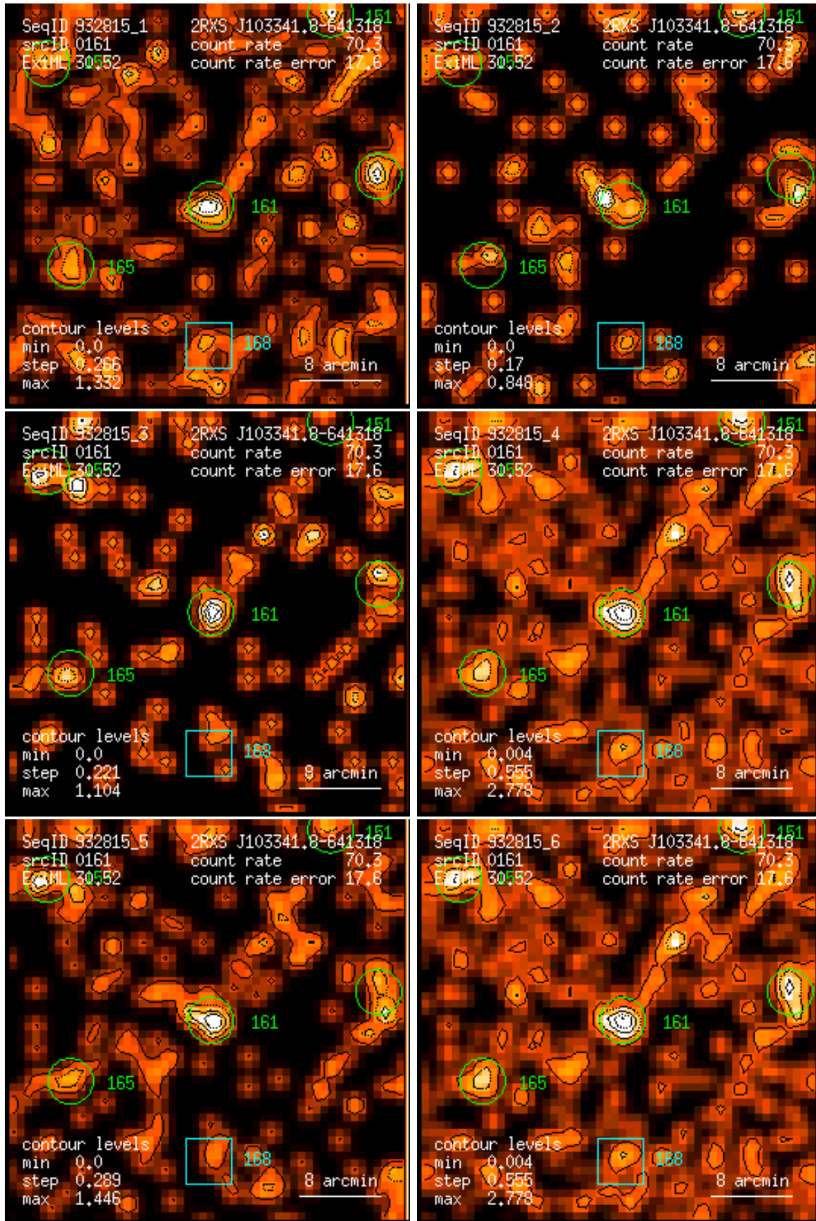
Figure 161: RASS 932815: detection 0161: band rate images, Gaussian filter: (1) PSPC channels 11 – 41, (2) 52 – 90, (3) 91 – 201, (4) 11 – 235, (5) 52 – 201, (6) 11 – 201. Broad band rates in counts/ks. Band rate contour levels in counts/ks/arcmin 2 .
