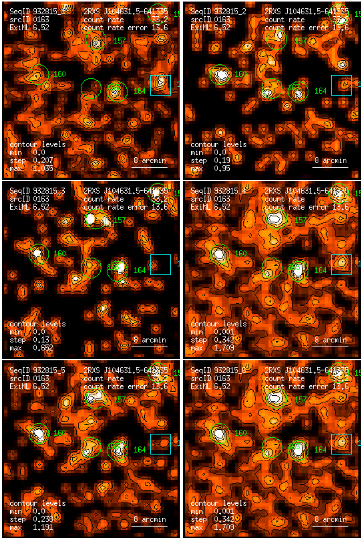
Figure 163: RASS 932815: detection 0163: band rate images, Gaussian filter: (1) PSPC channels 11 – 41, (2) 52 – 90, (3) 91 – 201, (4) 11 – 235, (5) 52 – 201, (6) 11 – 201. Broad band rates in counts/ks. Band rate contour levels in counts/ks/arcmin 2 .
