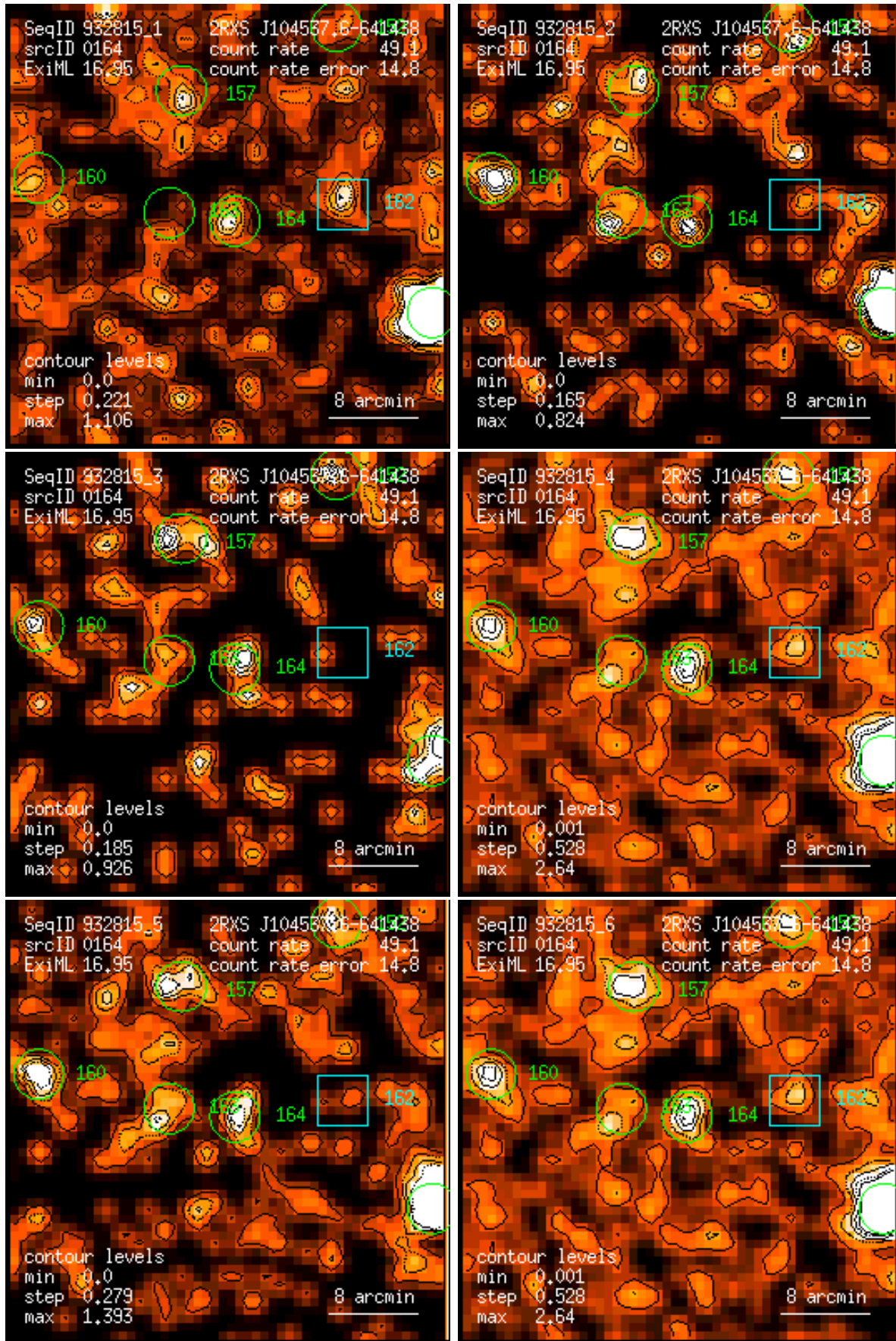
Figure 164: RASS 932815: detection 0164: band rate images, Gaussian filter: (1) PSPC channels 11 – 41, (2) 52 – 90, (3) 91 – 201, (4) 11 – 235, (5) 52 – 201, (6) 11 – 201. Broad band rates in counts/ks. Band rate contour levels in counts/ks/arcmin 2 .
