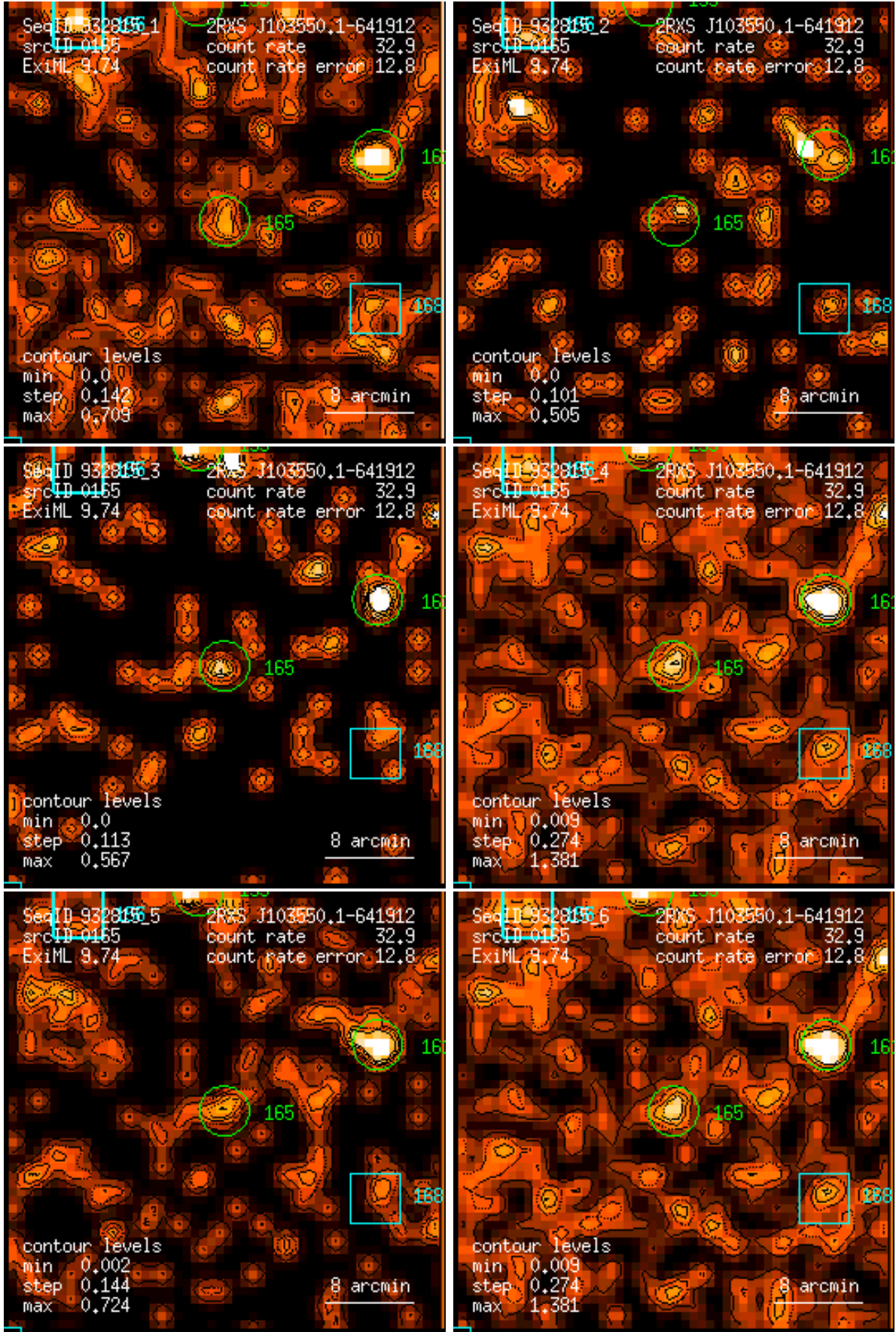
Figure 165: RASS 932815: detection 0165: band rate images, Gaussian filter: (1) PSPC channels 11 – 41, (2) 52 – 90, (3) 91 – 201, (4) 11 – 235, (5) 52 – 201, (6) 11 – 201. Broad band rates in counts/ks. Band rate contour levels in counts/ks/arcmin 2 .
