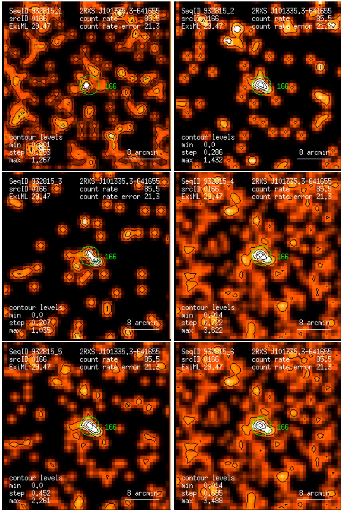
Figure 166: RASS 932815: detection 0166: band rate images, Gaussian filter: (1) PSPC channels 11 – 41, (2) 52 – 90, (3) 91 – 201, (4) 11 – 235, (5) 52 – 201, (6) 11 – 201. Broad band rates in counts/ks. Band rate contour levels in counts/ks/arcmin 2 .
