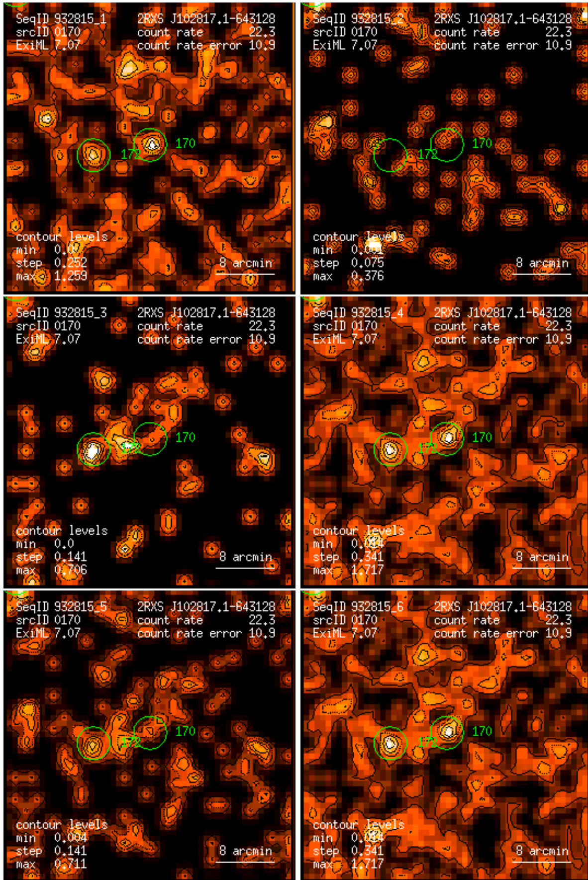
Figure 170: RASS 932815: detection 0170: band rate images, Gaussian filter: (1) PSPC channels 11 – 41, (2) 52 – 90, (3) 91 – 201, (4) 11 – 235, (5) 52 – 201, (6) 11 – 201. Broad band rates in counts/ks. Band rate contour levels in counts/ks/arcmin 2 .
