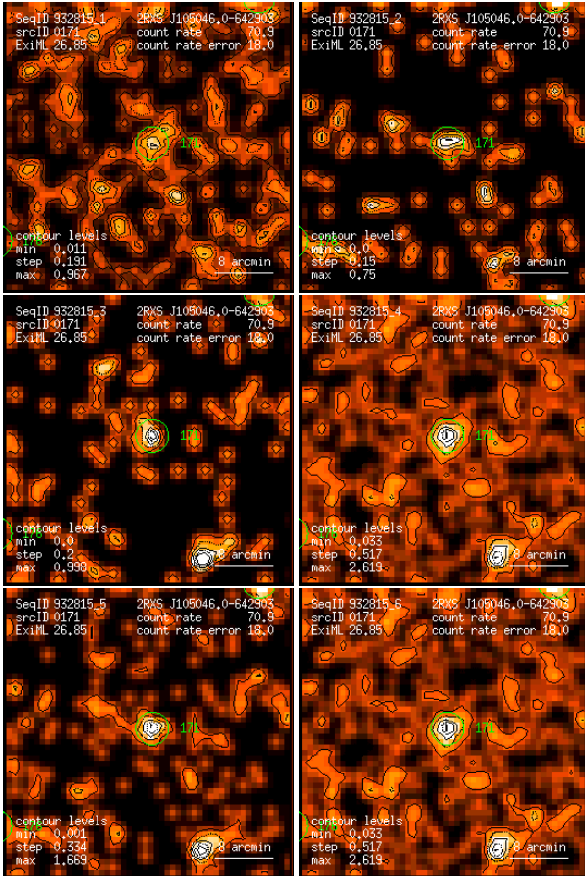
Figure 171: RASS 932815: detection 0171: band rate images, Gaussian filter: (1) PSPC channels 11 – 41, (2) 52 – 90, (3) 91 – 201, (4) 11 – 235, (5) 52 – 201, (6) 11 – 201. Broad band rates in counts/ks. Band rate contour levels in counts/ks/arcmin 2 .
