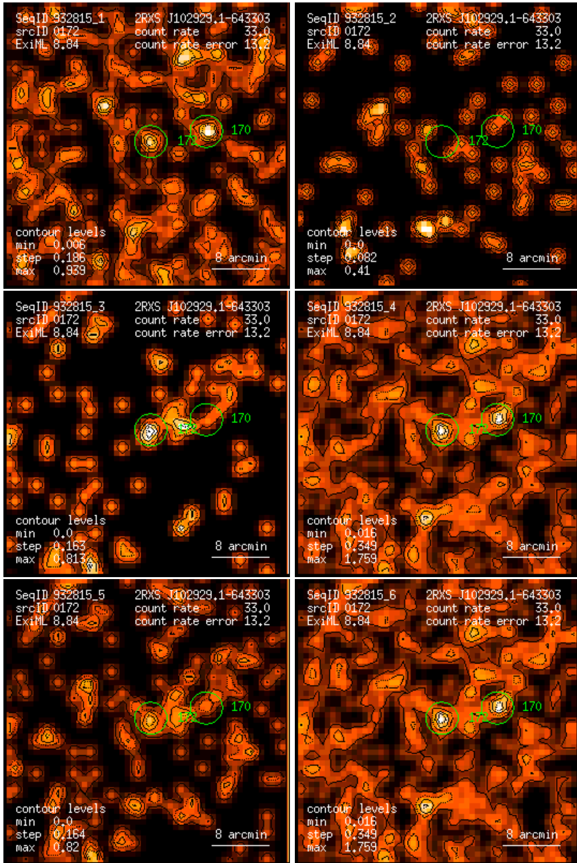
Figure 172: RASS 932815: detection 0172: band rate images, Gaussian filter: (1) PSPC channels 11 – 41, (2) 52 – 90, (3) 91 – 201, (4) 11 – 235, (5) 52 – 201, (6) 11 – 201. Broad band rates in counts/ks. Band rate contour levels in counts/ks/arcmin 2 .
