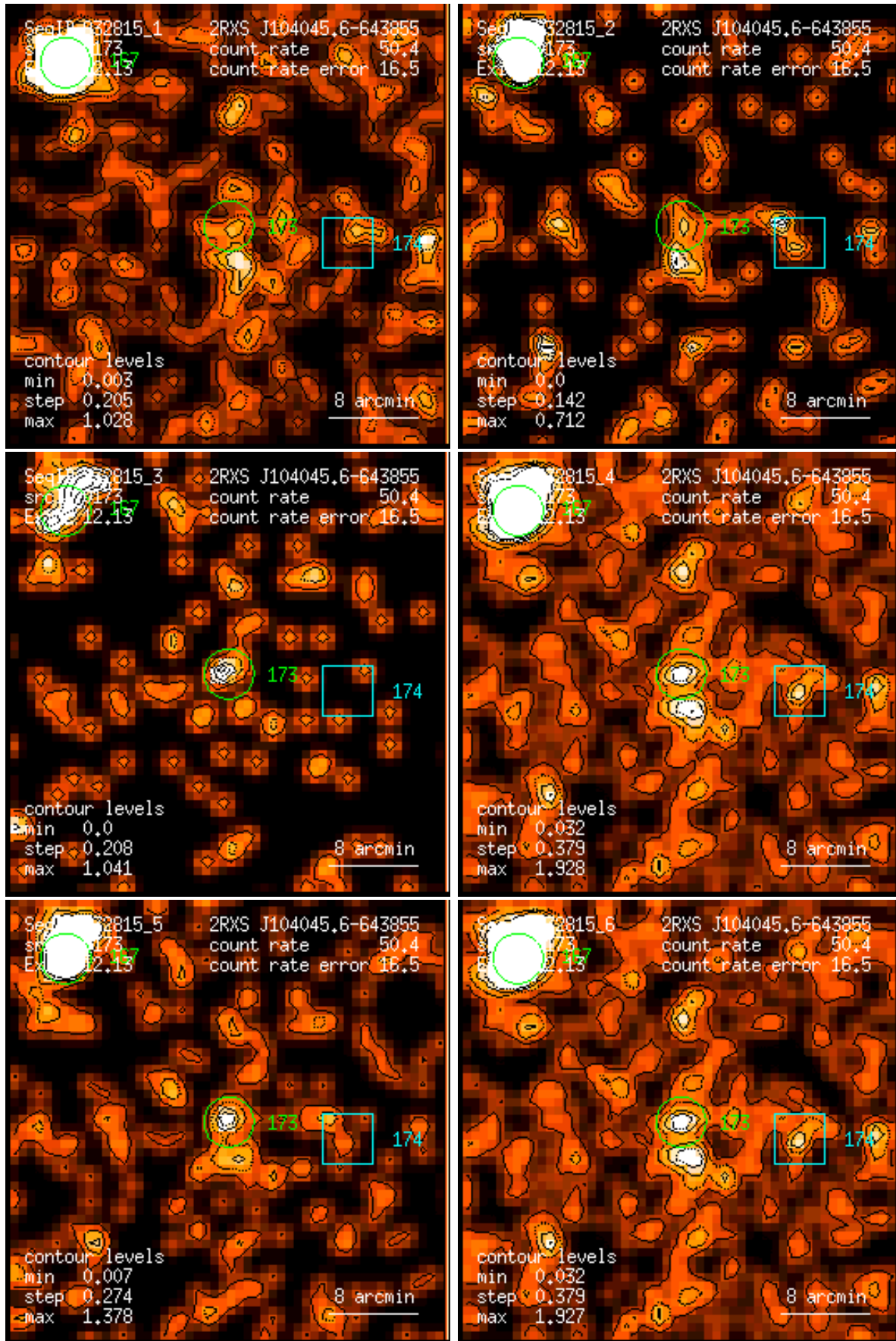
Figure 173: RASS 932815: detection 0173: band rate images, Gaussian filter: (1) PSPC channels 11 – 41, (2) 52 – 90, (3) 91 – 201, (4) 11 – 235, (5) 52 – 201, (6) 11 – 201. Broad band rates in counts/ks. Band rate contour levels in counts/ks/arcmin 2 .
