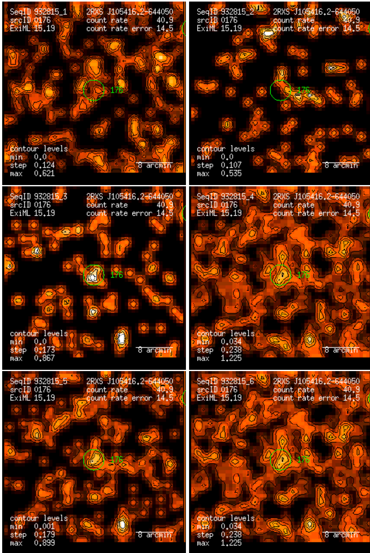
Figure 176: RASS 932815: detection 0176: band rate images, Gaussian filter: (1) PSPC channels 11 – 41, (2) 52 – 90, (3) 91 – 201, (4) 11 – 235, (5) 52 – 201, (6) 11 – 201. Broad band rates in counts/ks. Band rate contour levels in counts/ks/arcmin 2 .
