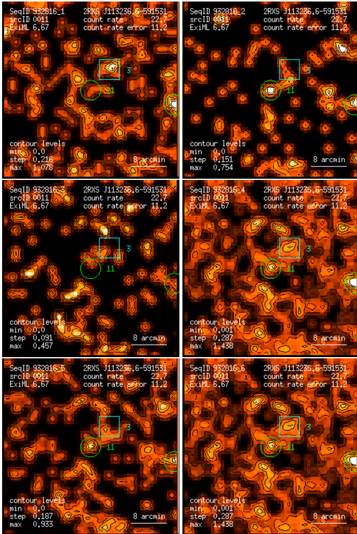
Figure 11: RASS 932816: detection 0011: band rate images, Gaussian filter: (1) PSPC channels 11 – 41, (2) 52 – 90, (3) 91 – 201, (4) 11 – 235, (5) 52 – 201, (6) 11 – 201. Broad band rates in counts/ks. Band rate contour levels in counts/ks/arcmin 2 .
