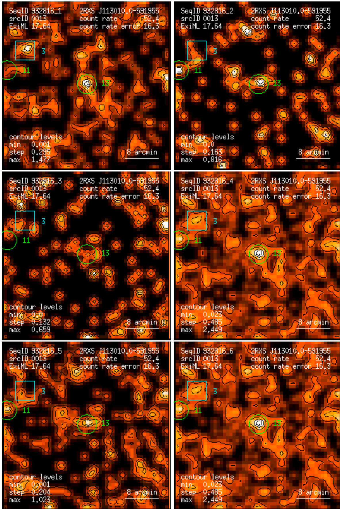
Figure 13: RASS 932816: detection 0013: band rate images, Gaussian filter: (1) PSPC channels 11 – 41, (2) 52 – 90, (3) 91 – 201, (4) 11 – 235, (5) 52 – 201, (6) 11 – 201. Broad band rates in counts/ks. Band rate contour levels in counts/ks/arcmin 2 .
