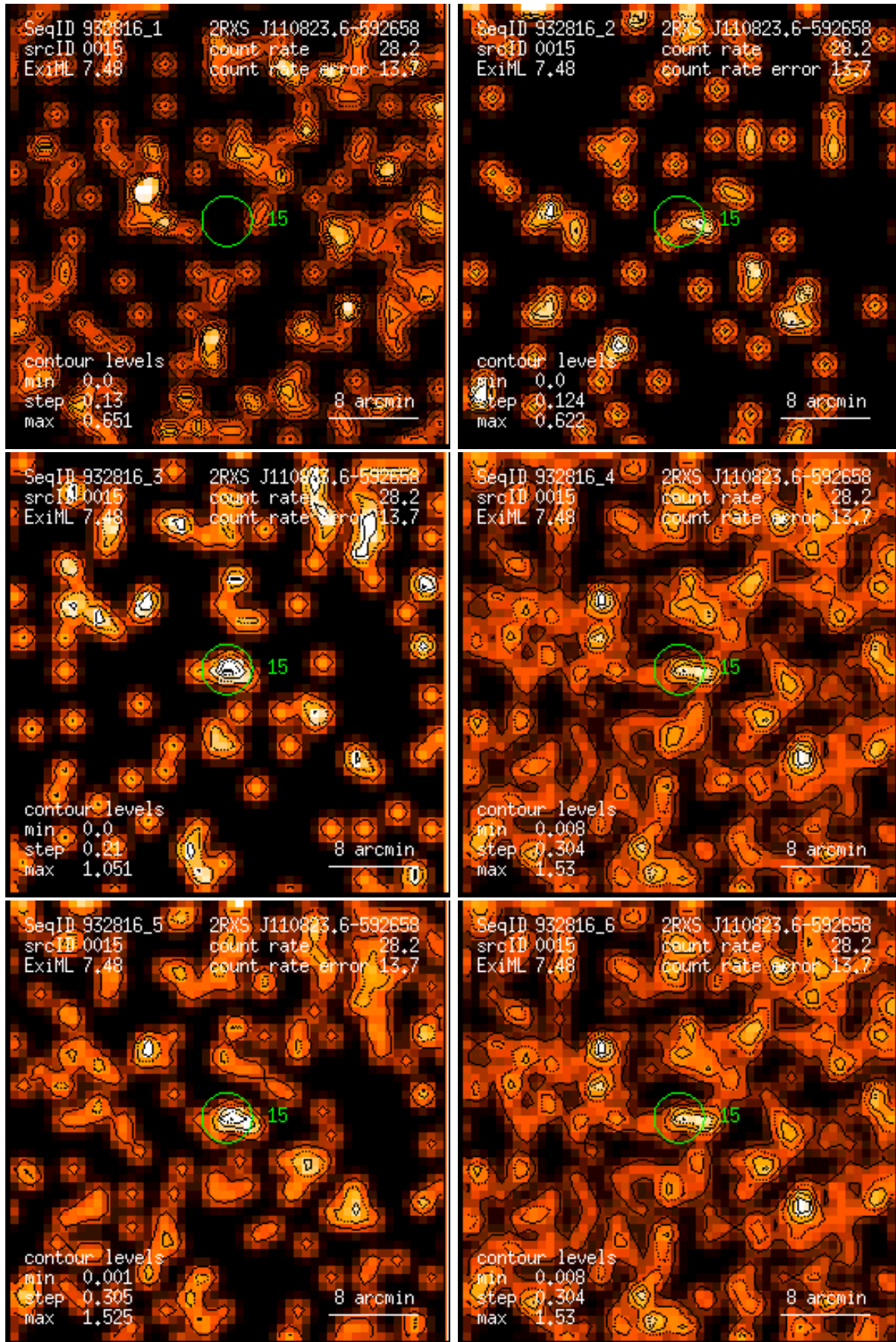
Figure 15: RASS 932816: detection 0015: band rate images, Gaussian filter: (1) PSPC channels 11 – 41, (2) 52 – 90, (3) 91 – 201, (4) 11 – 235, (5) 52 – 201, (6) 11 – 201. Broad band rates in counts/ks. Band rate contour levels in counts/ks/arcmin 2 .
