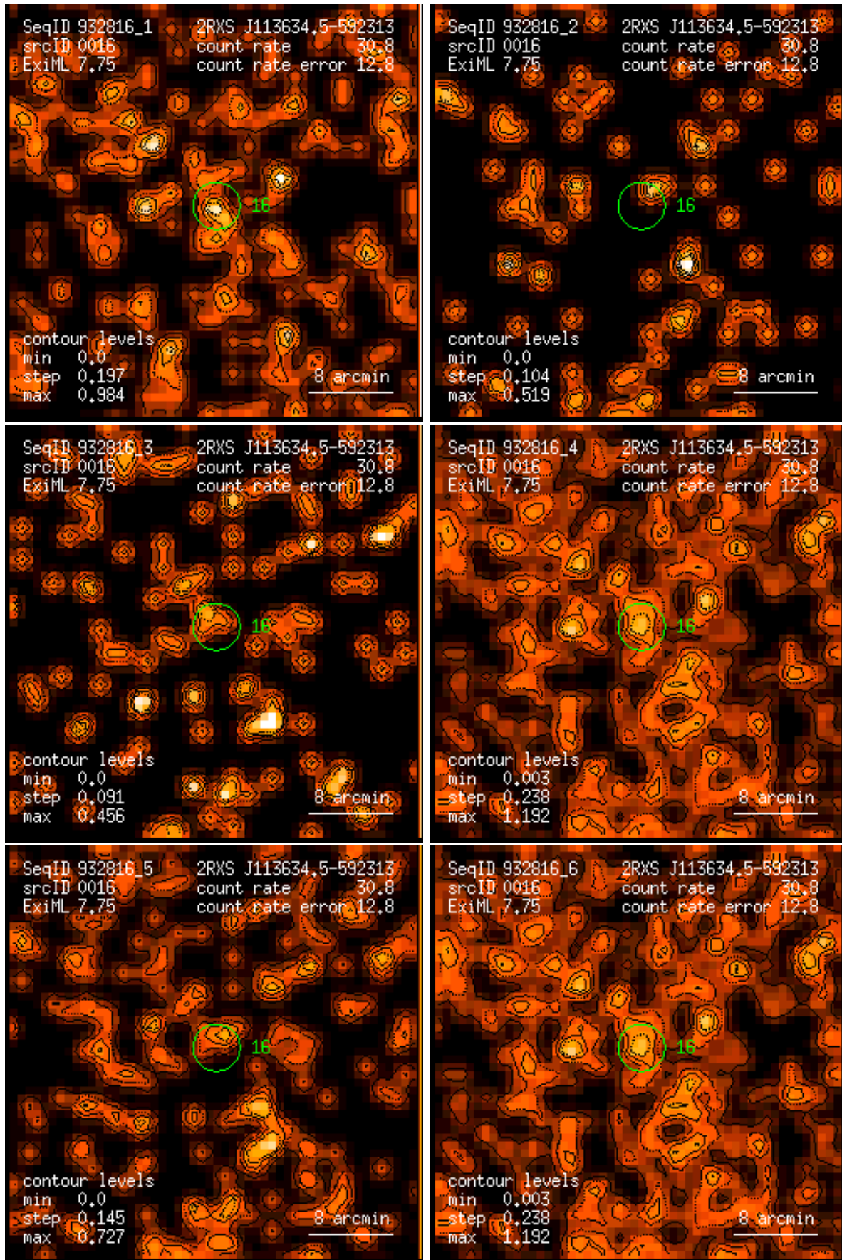
Figure 16: RASS 932816: detection 0016: band rate images, Gaussian filter: (1) PSPC channels 11 – 41, (2) 52 – 90, (3) 91 – 201, (4) 11 – 235, (5) 52 – 201, (6) 11 – 201. Broad band rates in counts/ks. Band rate contour levels in counts/ks/arcmin 2 .
