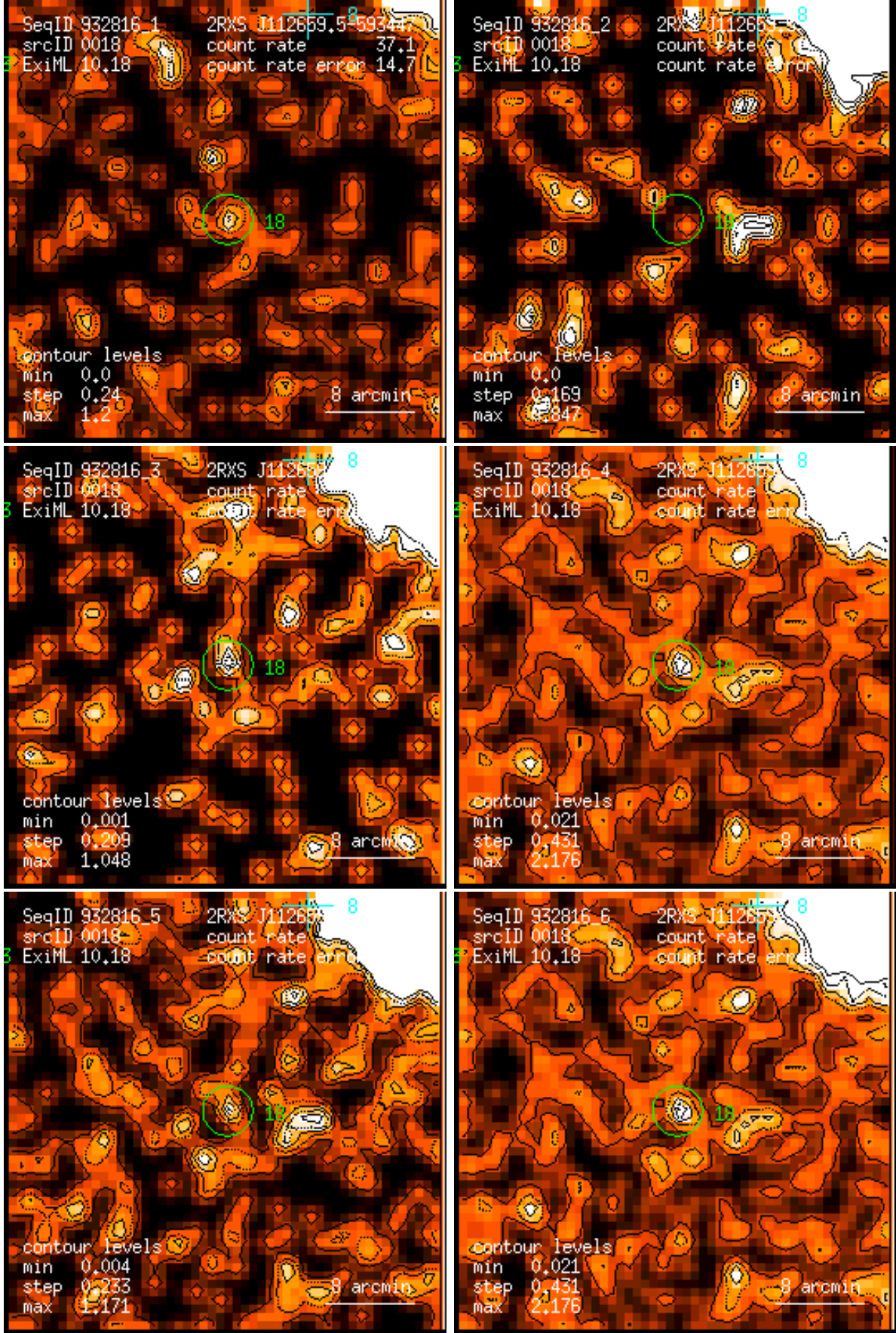
Figure 18: RASS 932816: detection 0018: band rate images, Gaussian filter: (1) PSPC channels 11 – 41, (2) 52 – 90, (3) 91 – 201, (4) 11 – 235, (5) 52 – 201, (6) 11 – 201. Broad band rates in counts/ks. Band rate contour levels in counts/ks/arcmin 2 .
