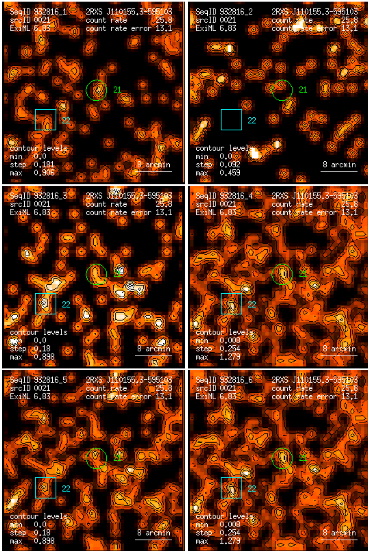
Figure 21: RASS 932816: detection 0021: band rate images, Gaussian filter: (1) PSPC channels 11 – 41, (2) 52 – 90, (3) 91 – 201, (4) 11 – 235, (5) 52 – 201, (6) 11 – 201. Broad band rates in counts/ks. Band rate contour levels in counts/ks/arcmin 2 .
