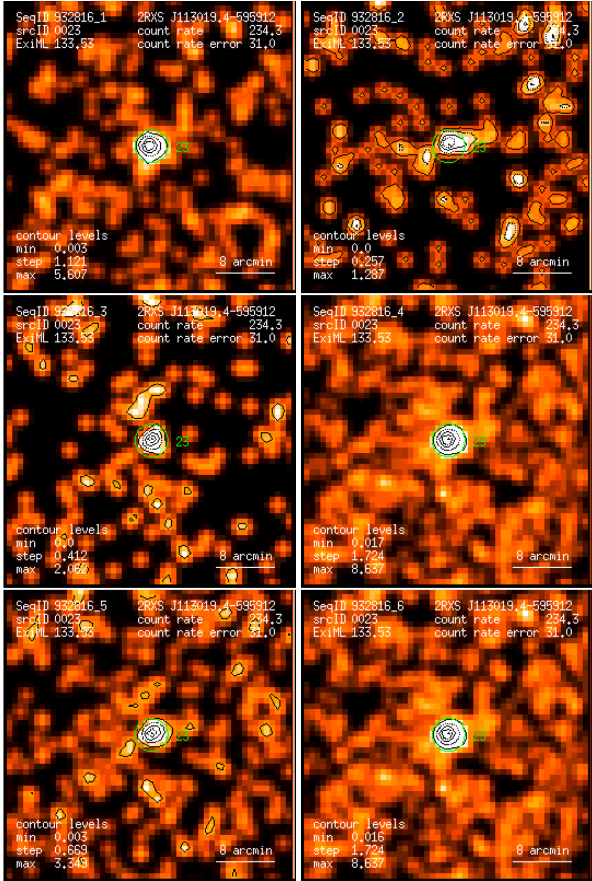
Figure 23: RASS 932816: detection 0023: band rate images, Gaussian filter: (1) PSPC channels 11 – 41, (2) 52 – 90, (3) 91 – 201, (4) 11 – 235, (5) 52 – 201, (6) 11 – 201. Broad band rates in counts/ks. Band rate contour levels in counts/ks/arcmin 2 .
