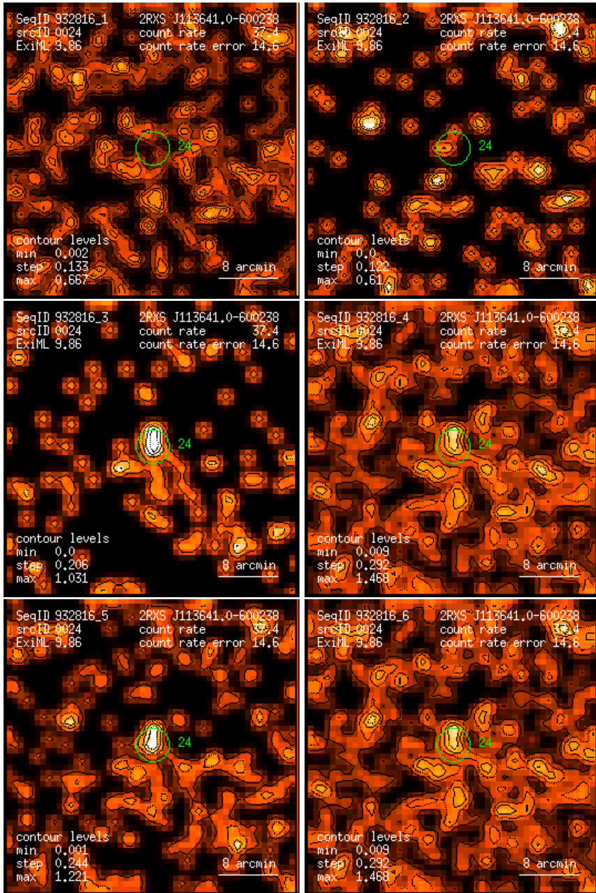
Figure 24: RASS 932816: detection 0024: band rate images, Gaussian filter: (1) PSPC channels 11 – 41, (2) 52 – 90, (3) 91 – 201, (4) 11 – 235, (5) 52 – 201, (6) 11 – 201. Broad band rates in counts/ks. Band rate contour levels in counts/ks/arcmin 2 .
