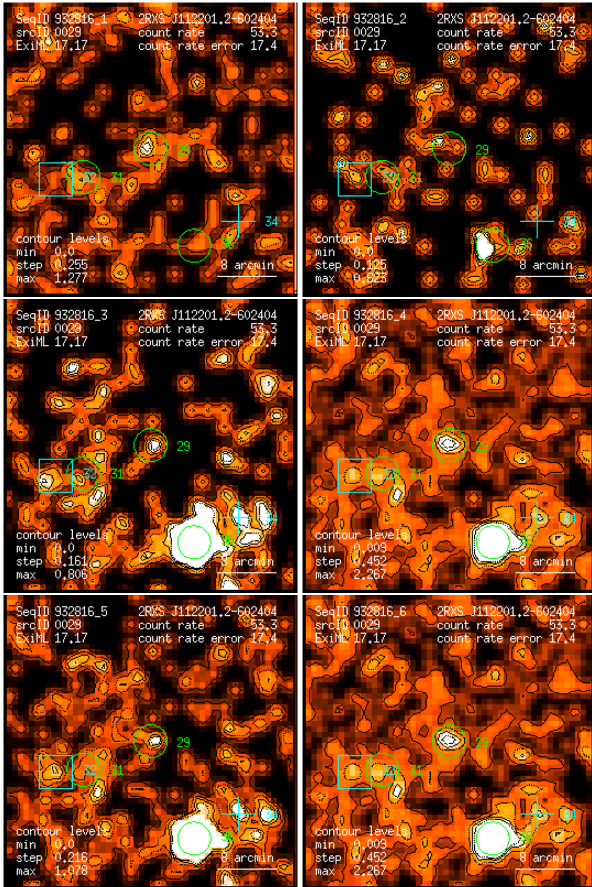
Figure 29: RASS 932816: detection 0029: band rate images, Gaussian filter: (1) PSPC channels 11 – 41, (2) 52 – 90, (3) 91 – 201, (4) 11 – 235, (5) 52 – 201, (6) 11 – 201. Broad band rates in counts/ks. Band rate contour levels in counts/ks/arcmin 2 .
