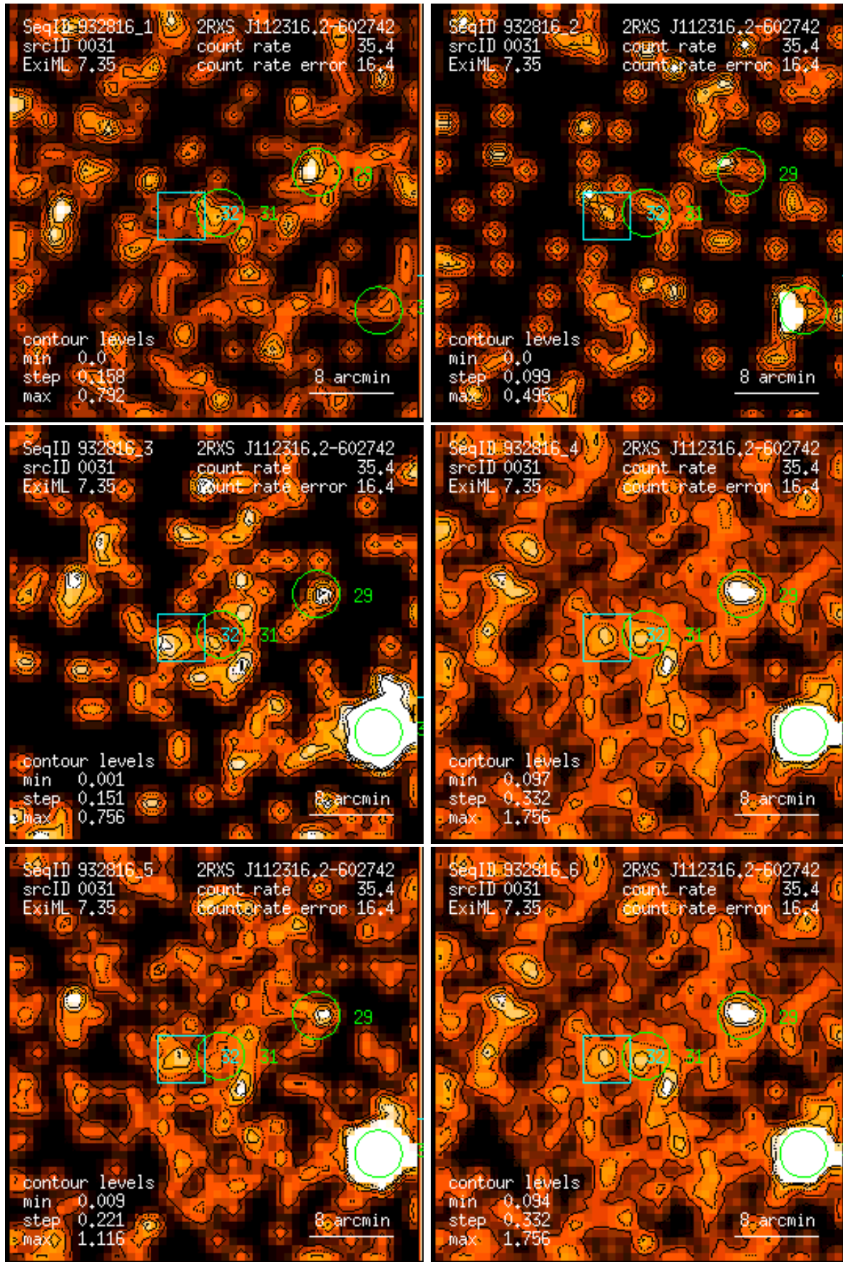
Figure 31: RASS 932816: detection 0031: band rate images, Gaussian filter: (1) PSPC channels 11 – 41, (2) 52 – 90, (3) 91 – 201, (4) 11 – 235, (5) 52 – 201, (6) 11 – 201. Broad band rates in counts/ks. Band rate contour levels in counts/ks/arcmin 2 .
