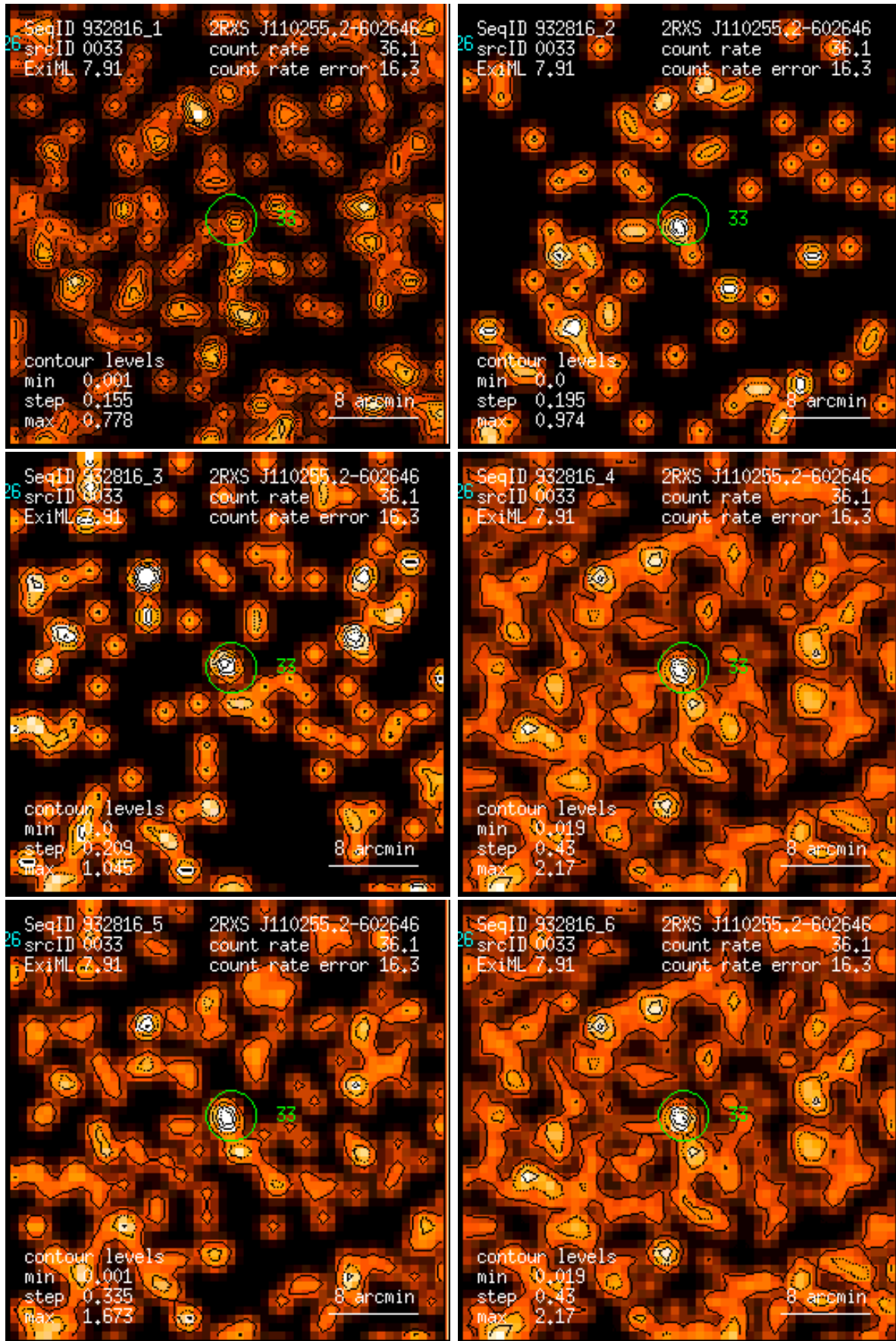
Figure 33: RASS 932816: detection 0033: band rate images, Gaussian filter: (1) PSPC channels 11 – 41, (2) 52 – 90, (3) 91 – 201, (4) 11 – 235, (5) 52 – 201, (6) 11 – 201. Broad band rates in counts/ks. Band rate contour levels in counts/ks/arcmin 2 .
