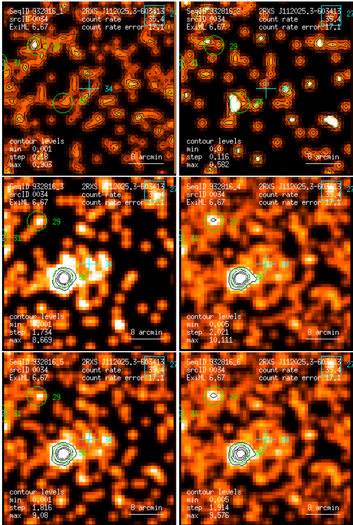
Figure 34: RASS 932816: detection 0034: band rate images, Gaussian filter: (1) PSPC channels 11 – 41, (2) 52 – 90, (3) 91 – 201, (4) 11 – 235, (5) 52 – 201, (6) 11 – 201. Broad band rates in counts/ks. Band rate contour levels in counts/ks/arcmin 2 .
