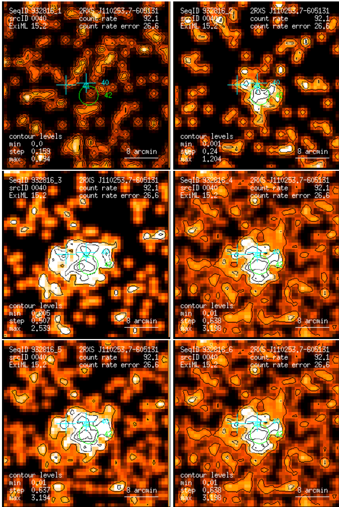
Figure 40: RASS 932816: detection 0040: band rate images, Gaussian filter: (1) PSPC channels 11 – 41, (2) 52 – 90, (3) 91 – 201, (4) 11 – 235, (5) 52 – 201, (6) 11 – 201. Broad band rates in counts/ks. Band rate contour levels in counts/ks/arcmin 2 .
