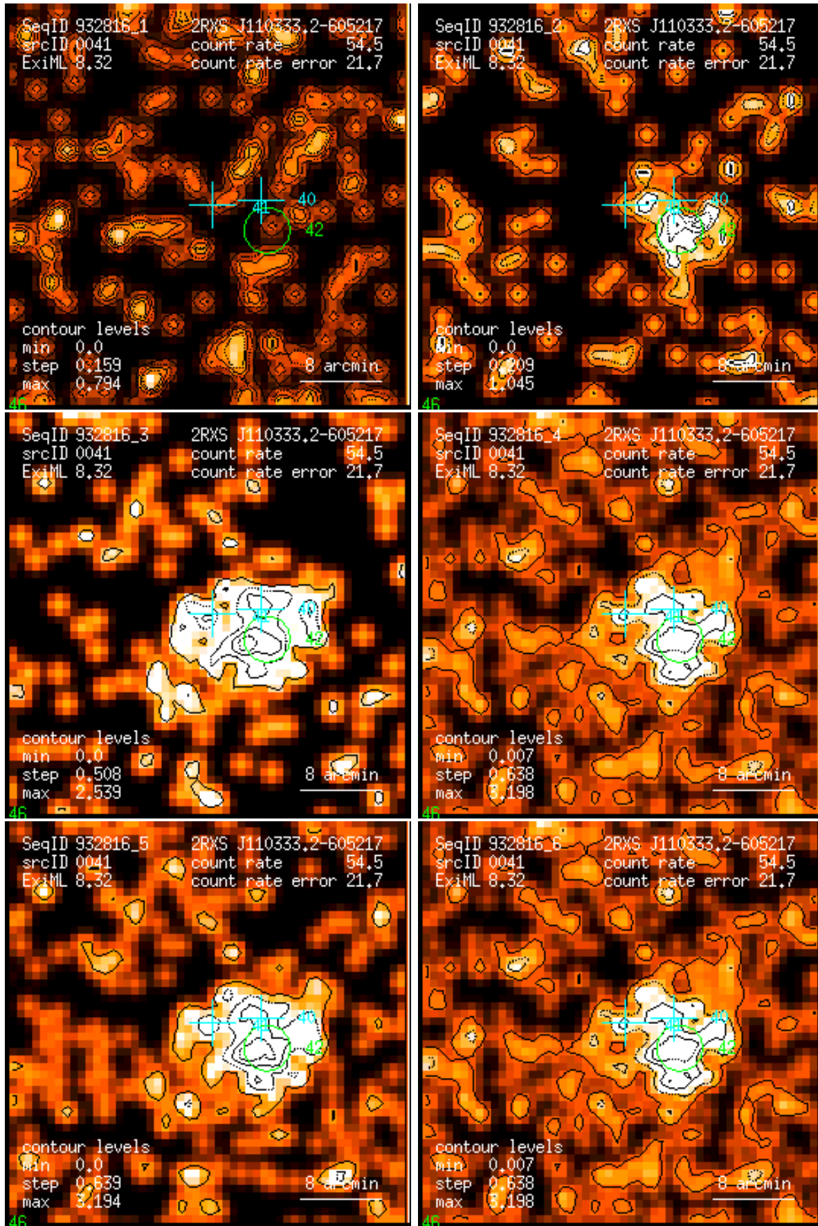
Figure 41: RASS 932816: detection 0041: band rate images, Gaussian filter: (1) PSPC channels 11 – 41, (2) 52 – 90, (3) 91 – 201, (4) 11 – 235, (5) 52 – 201, (6) 11 – 201. Broad band rates in counts/ks. Band rate contour levels in counts/ks/arcmin 2 .
